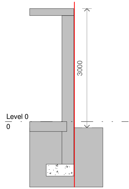
3 Prior Approval Section 1 : 50
