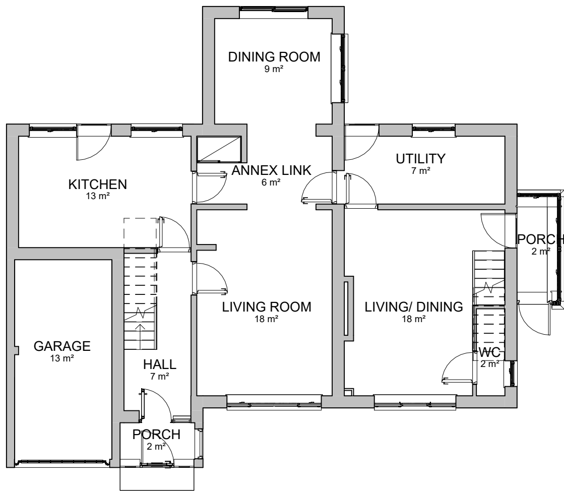
1 Existing Ground Floor Plan 1 : 100
