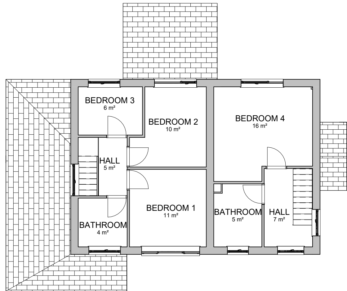
2 Existing First Floor Plan 1 : 100
