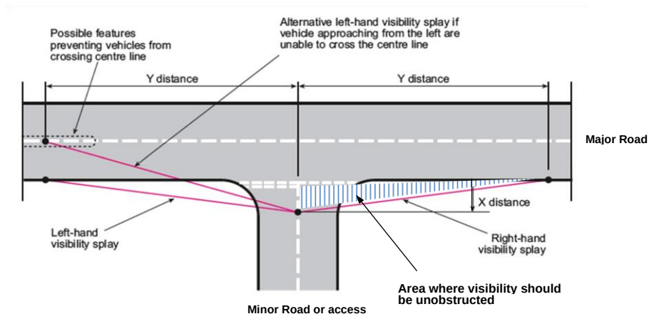
Figure b Visibility splay requirements
