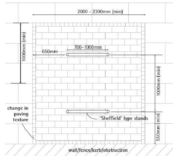
Cycle Parking Stand footprint (plan view)
