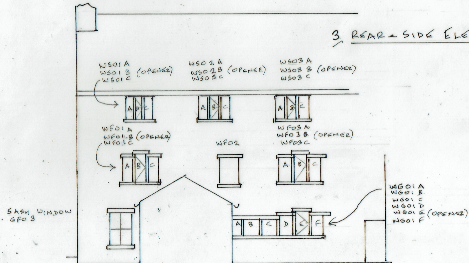
EXISTING REAR
