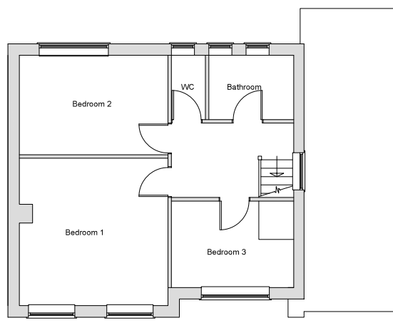
EXISTING 1st. FLOOR PLAN
