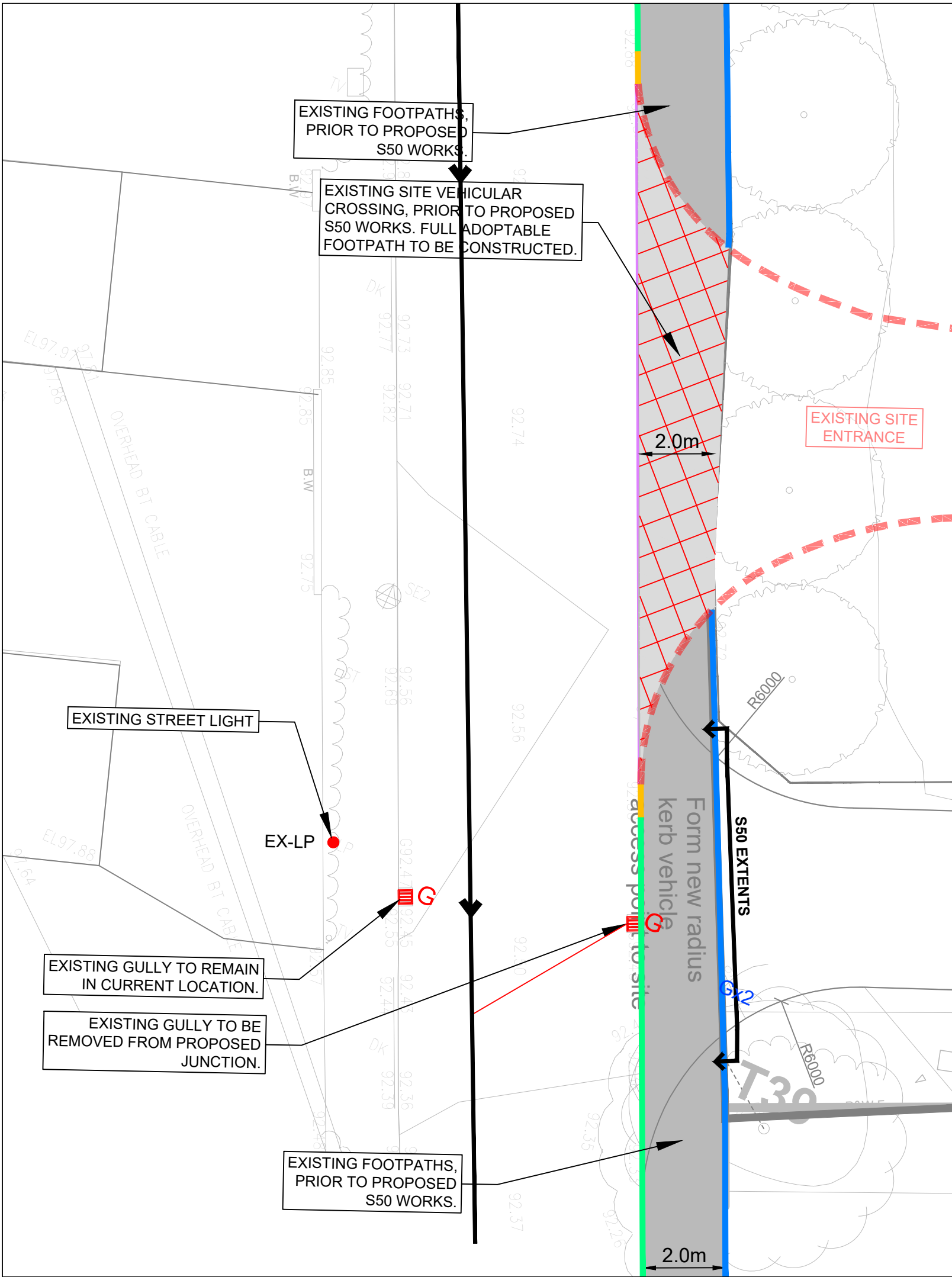
EXISTING SITE ENTRANCE PRIOR TO S50 WORKS SCALE: 1:125
