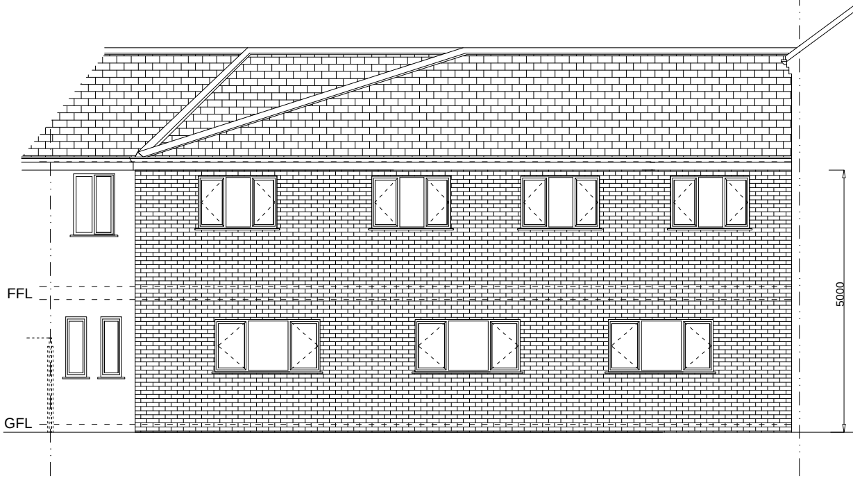
Proposed Rear Elevation As Amended
