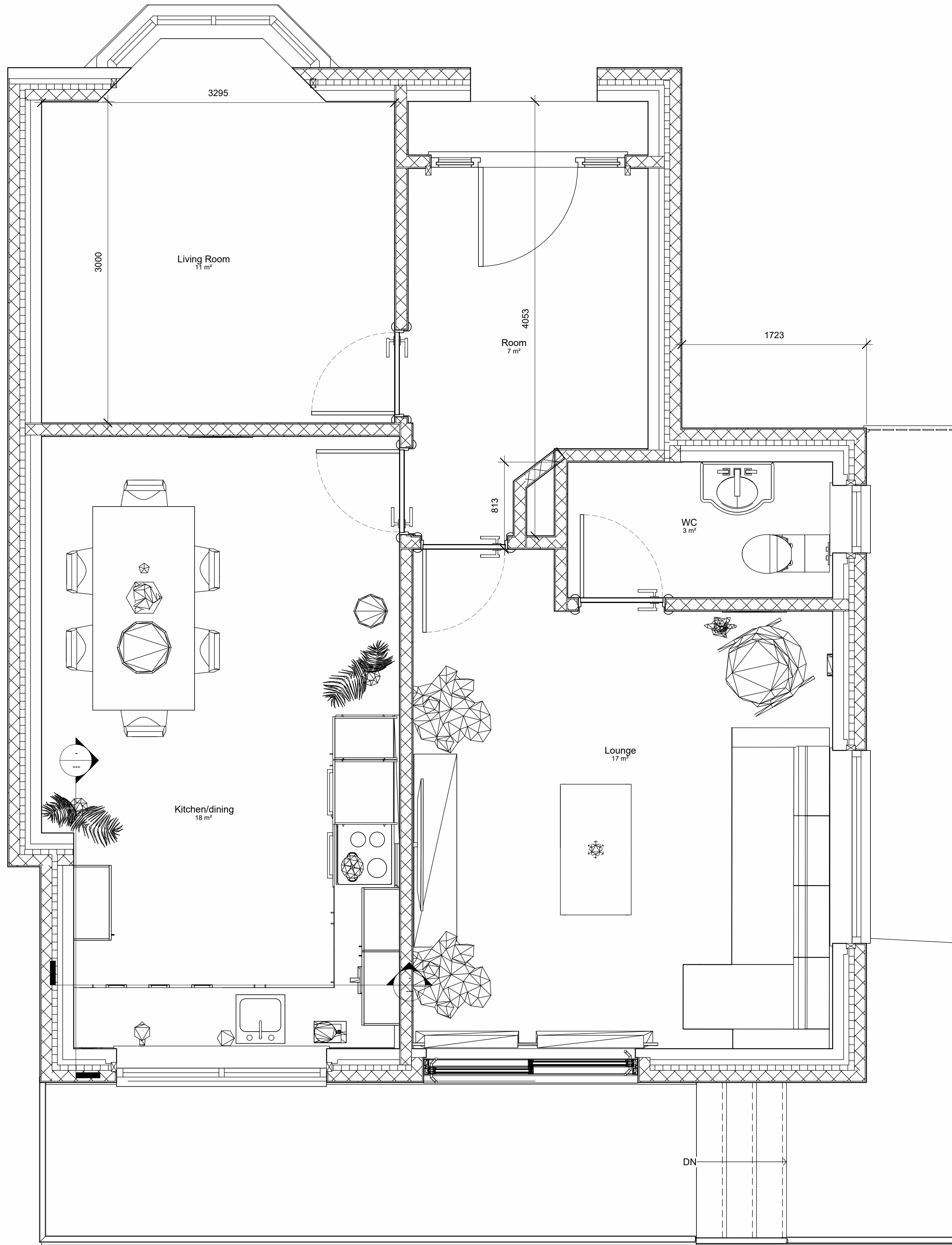
Ground Floor Plan 1 : 25
