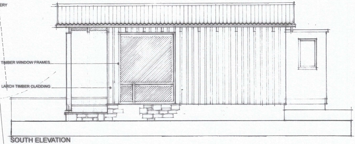
ELEVATIONS @ 1: 50 & 1: 100
