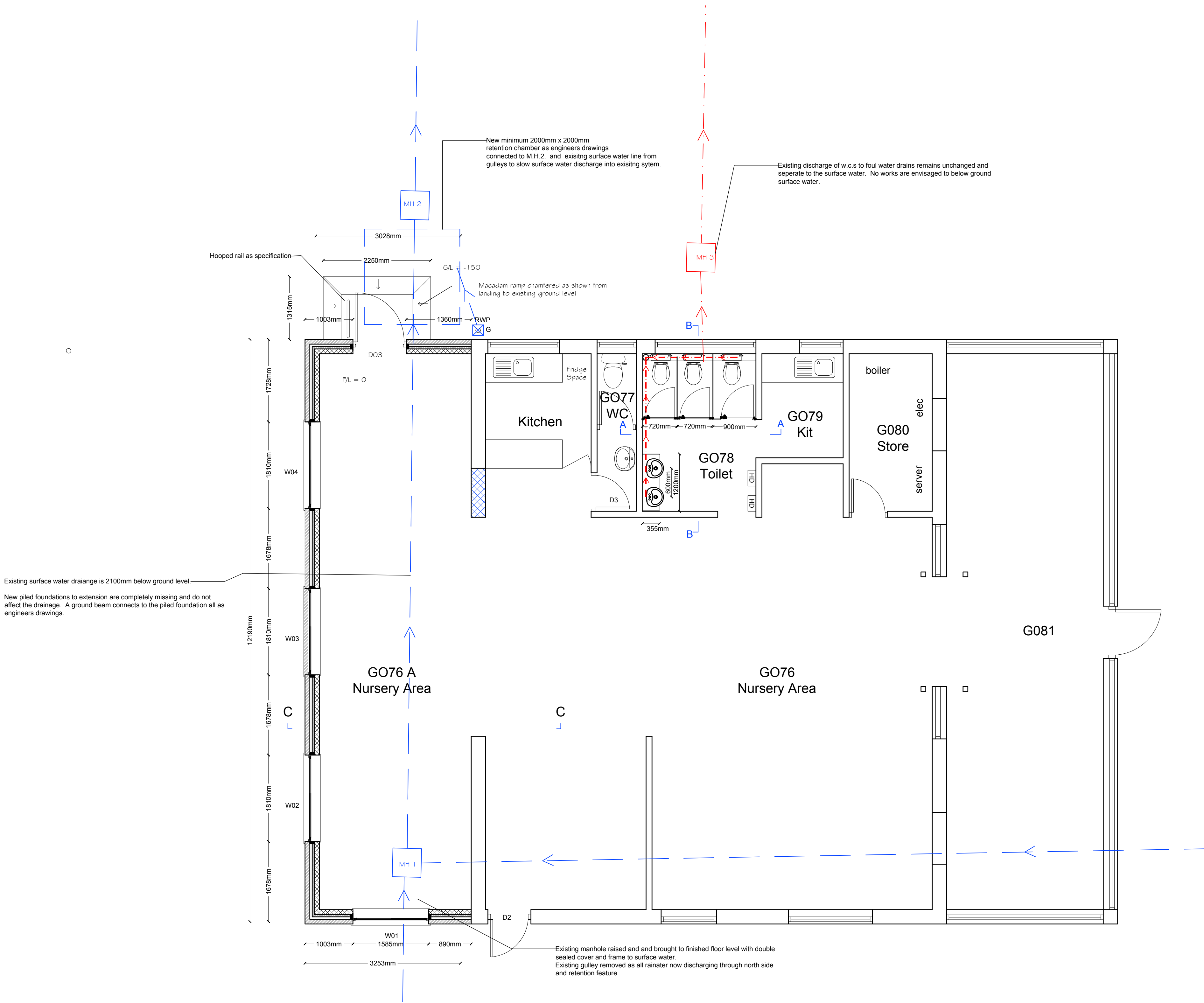
Proposed Layout Plan 1:50 @A1
