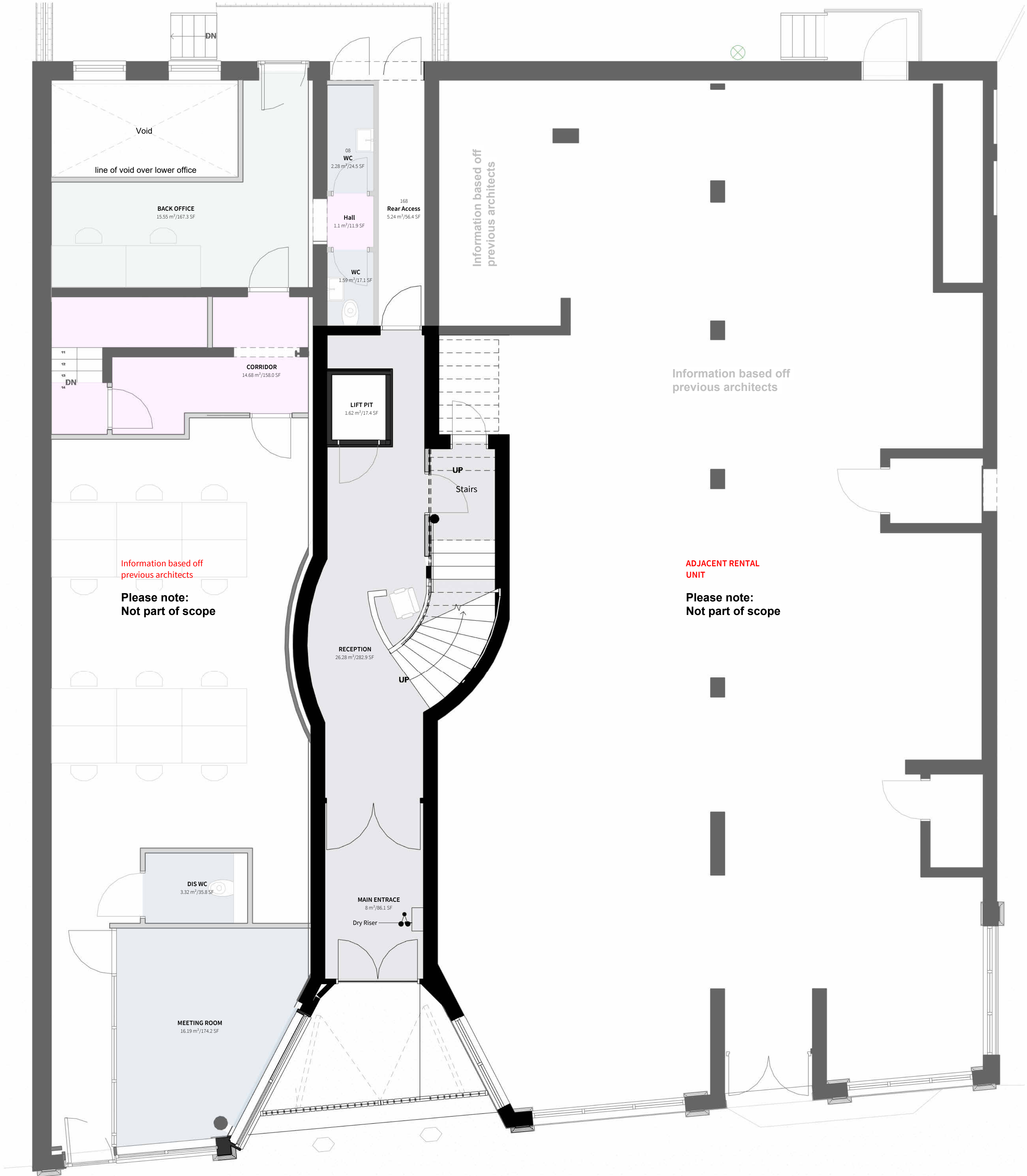
2 PROPOSED - GROUND FLOOR PLAN 1:50
