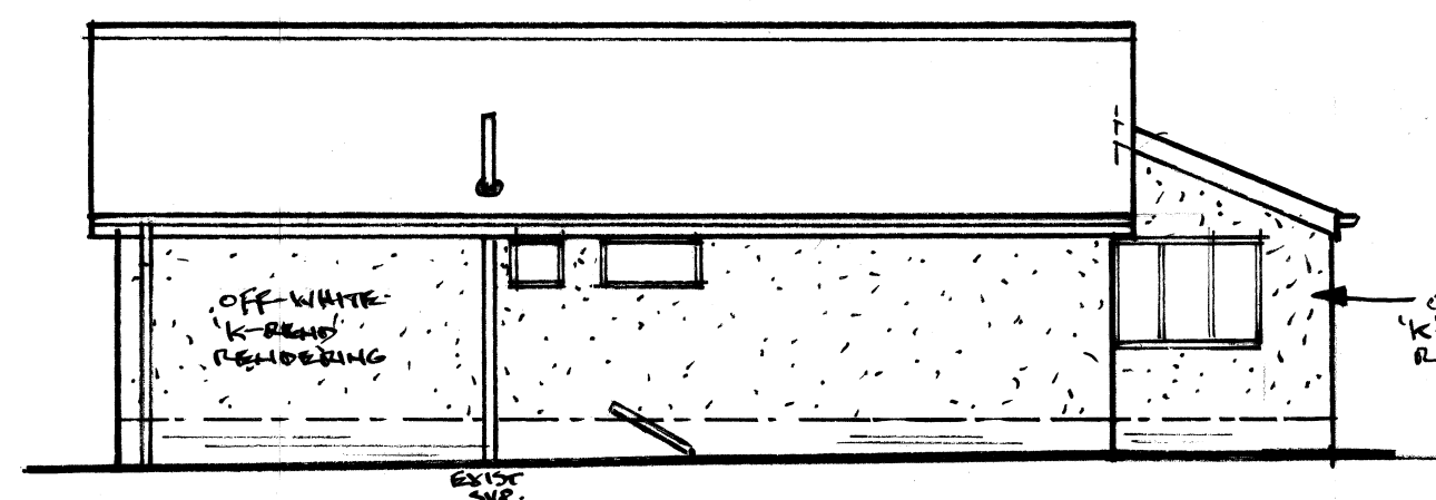
PROPOSED L.H. SIDE ELEVATION.
