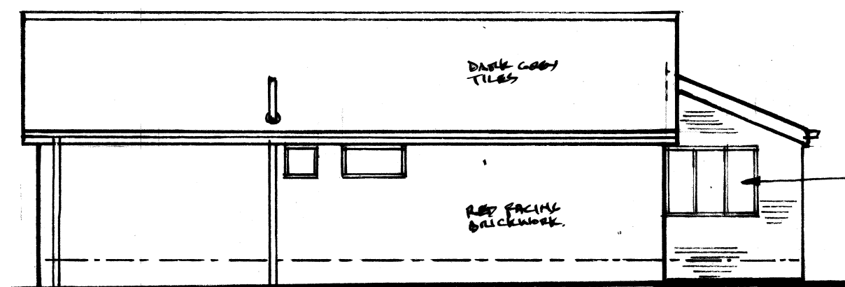
EXISTING L.H. SIDE ELEVATION. 1:100
