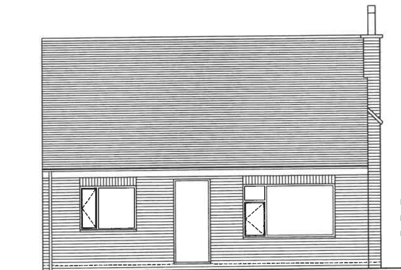
EXISTING FRONT ELEVATION 1:100 @ A4
