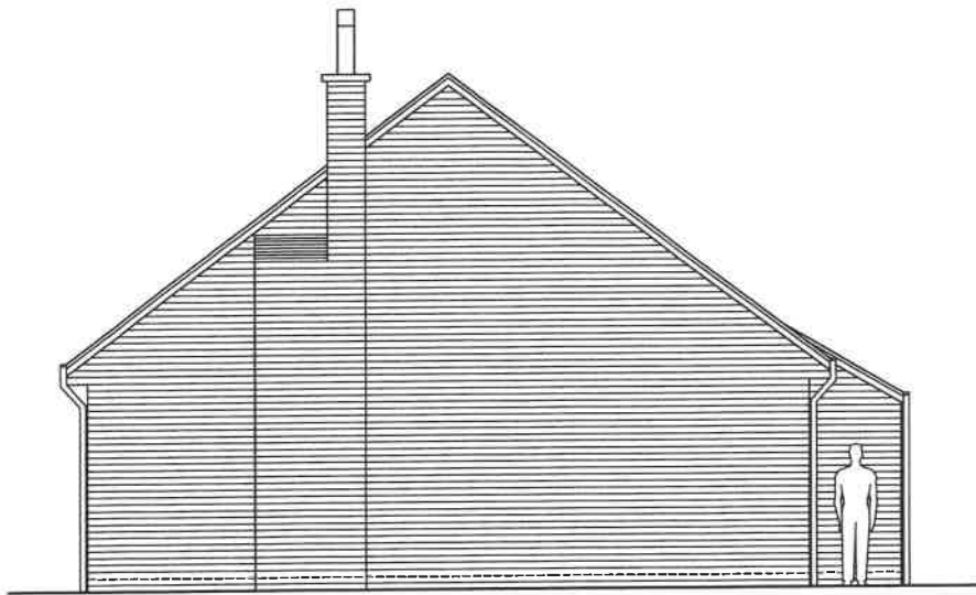
PROPOSED SIDE ELEVATION [VIEWED FROM NO. 880] 1:100 @ A4
