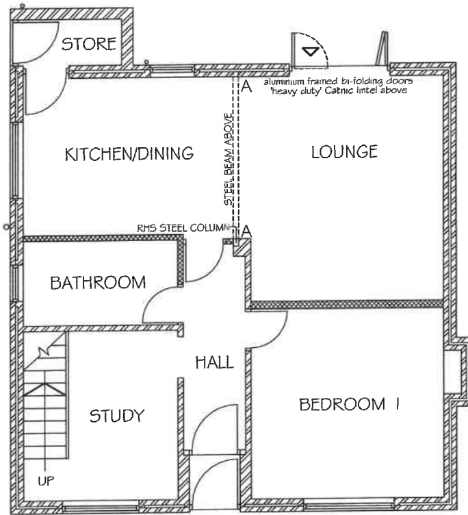
PROPOSED GROUND FLOOR LAYOUT 1:100 @ A4
