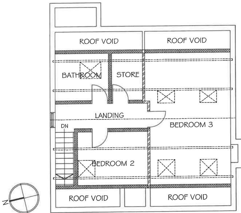
PROPOSED FIRST FLOOR LAYOUT 1:100 @ A4
