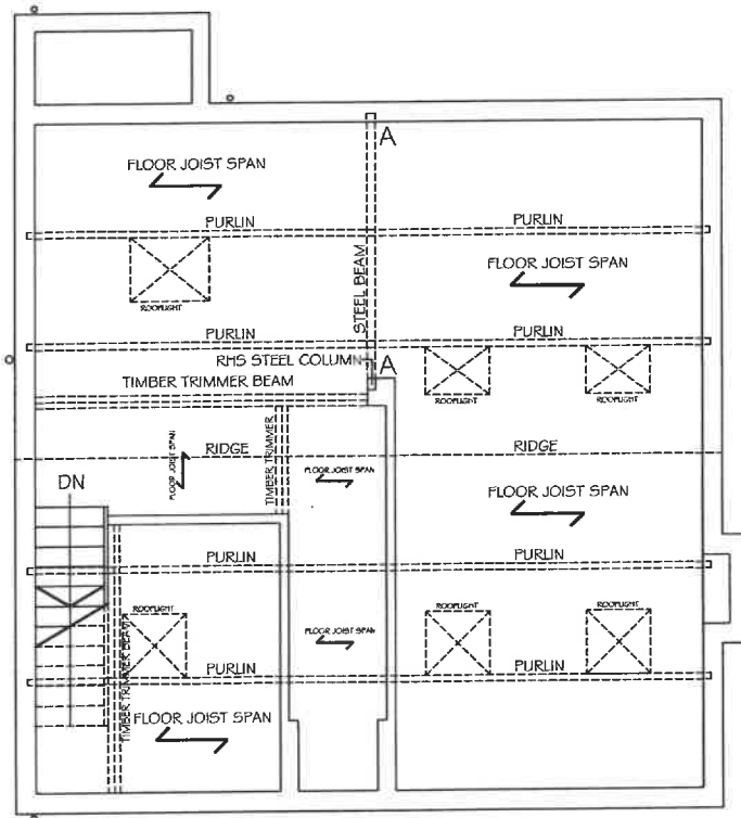
PROPOSED FIRST FLOOR STRUCTURE 1:100 @ A4
