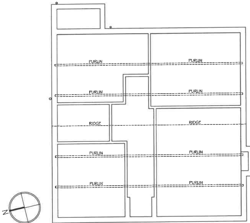
EXISTING ROOF STRUCTURE LAYOUT 1:100 @ A4
