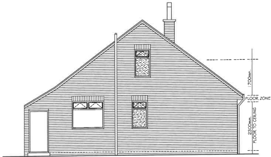
PROPOSED SIDE ELEVATION 1:100 @ A4
