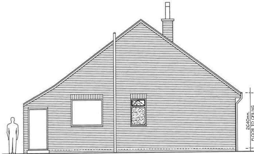
EXISTING SIDE ELEVATION 1:100 @ A4
