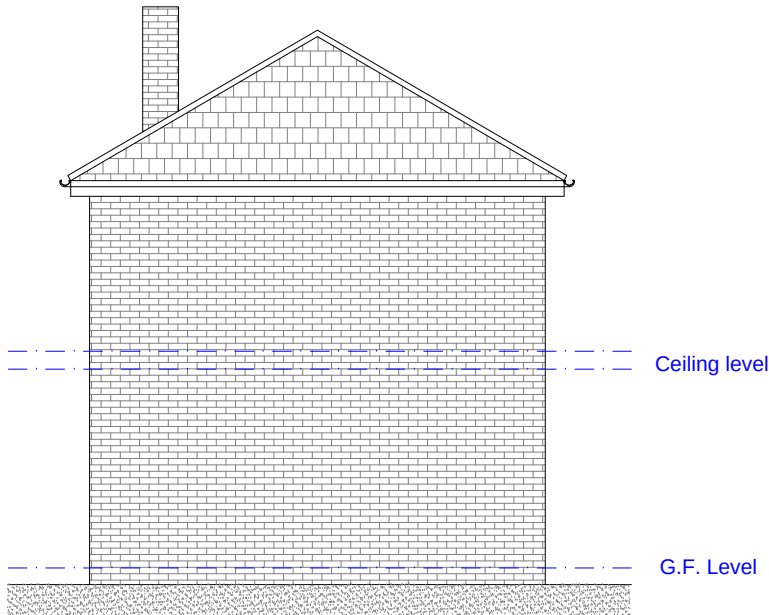
Existing L/H Side Elevation Scale 1:100
