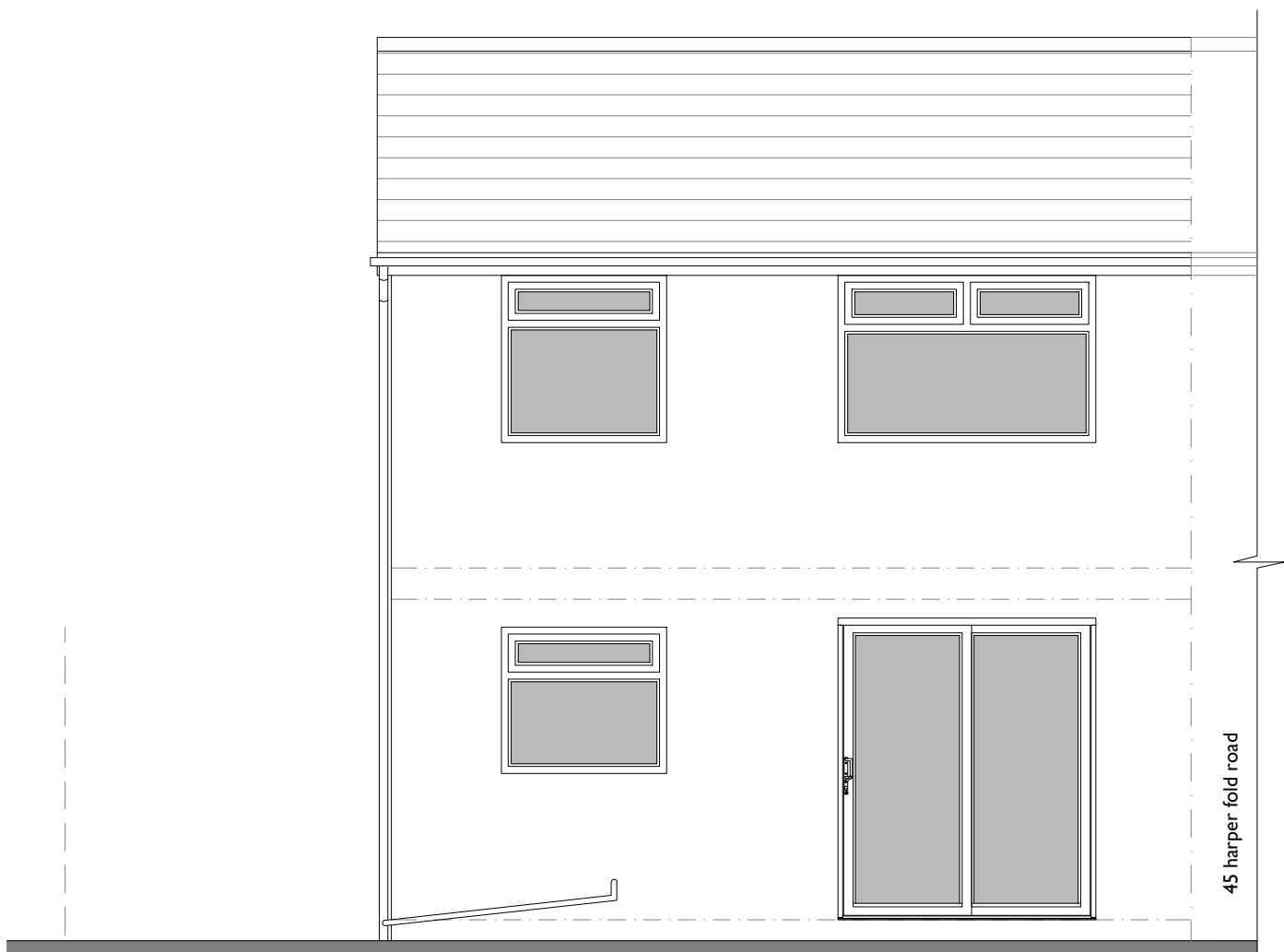
rear elevation (south)
