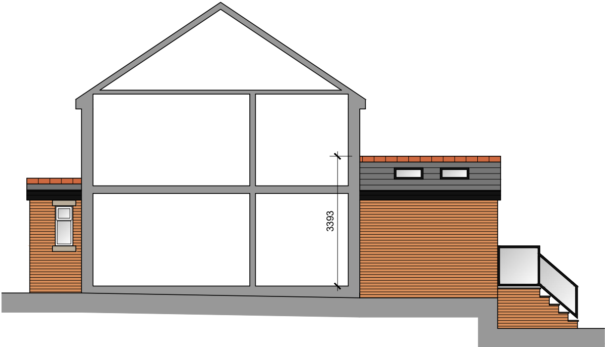
South West Facing Side Elevation
