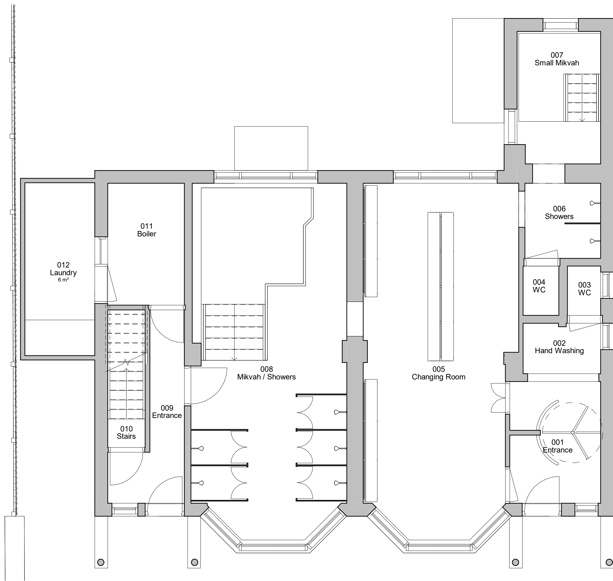
5. Level 0 - GA Existing 1 : 50
