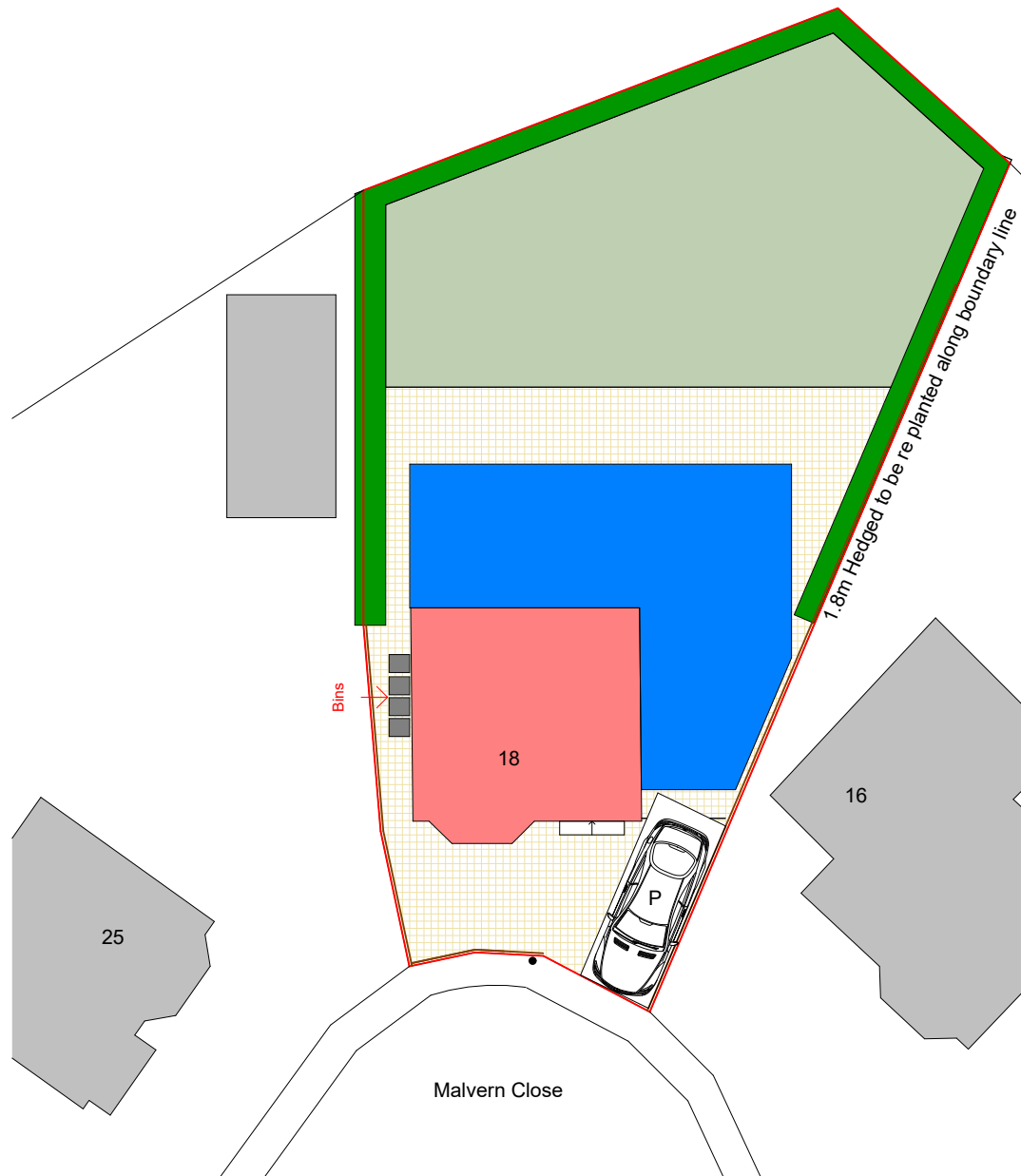
2 Site - Proposed 1 : 200
