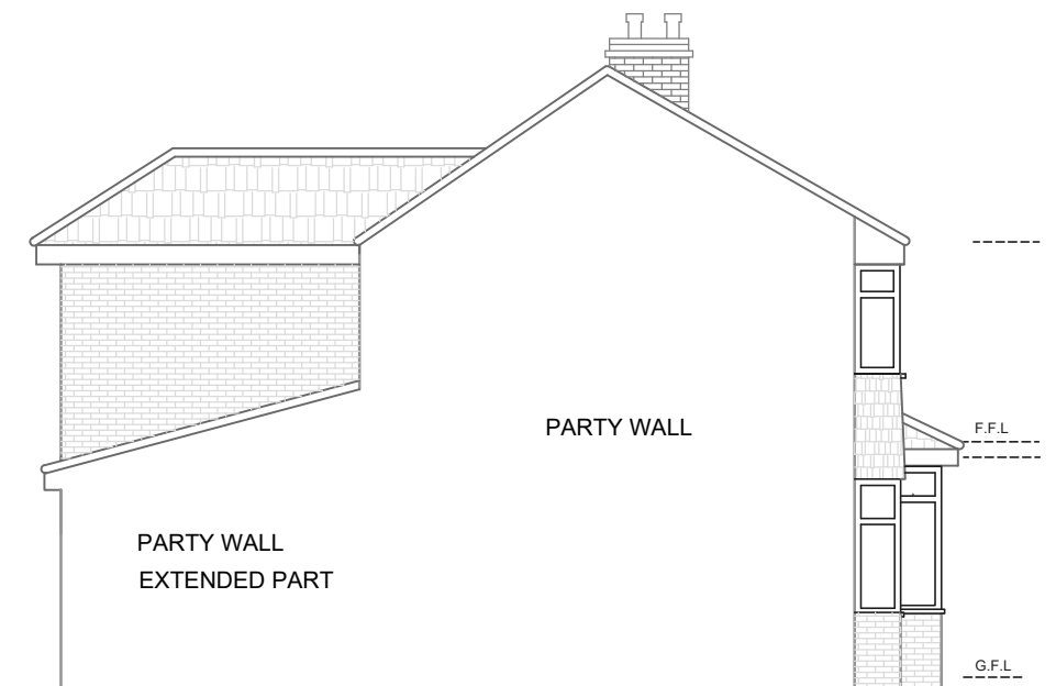
PROPOSED SIDE ELEVATION (NORTH EAST)
