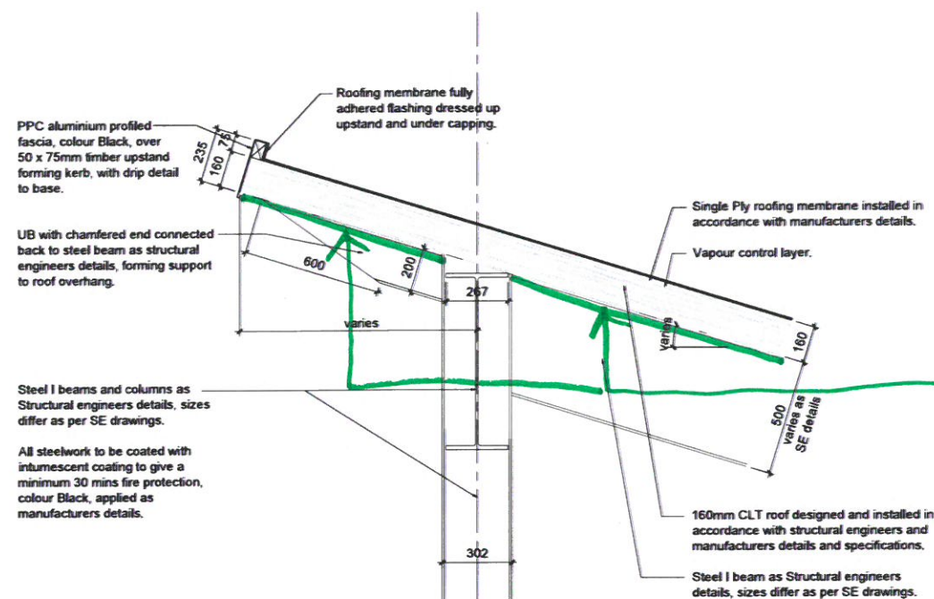
DETAIL 4 SINGLE PLY MEMBRANE CANOPY ROOF EDGE DETAIL
