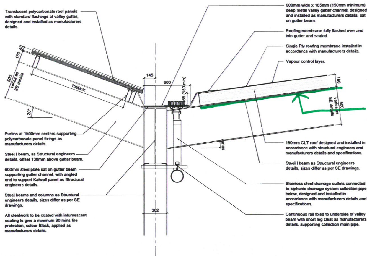
DETAIL 3 SINGLE PLY MEMBRANE & POLYCARBONATE PANEL CANOPY ROOF GUTTER DETAIL
