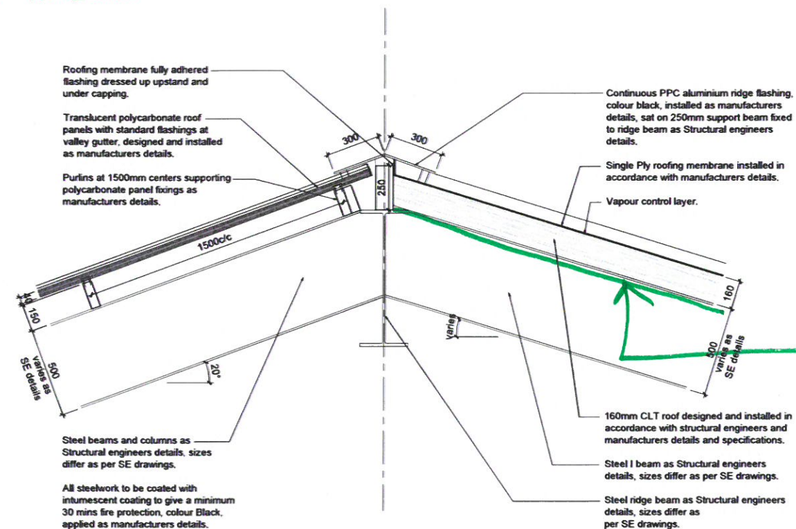
DETAIL 5 SINGLE PLY MEMBRANE & POLYCARBONATE PANEL CANOPY ROOF RIDGE DETAIL
