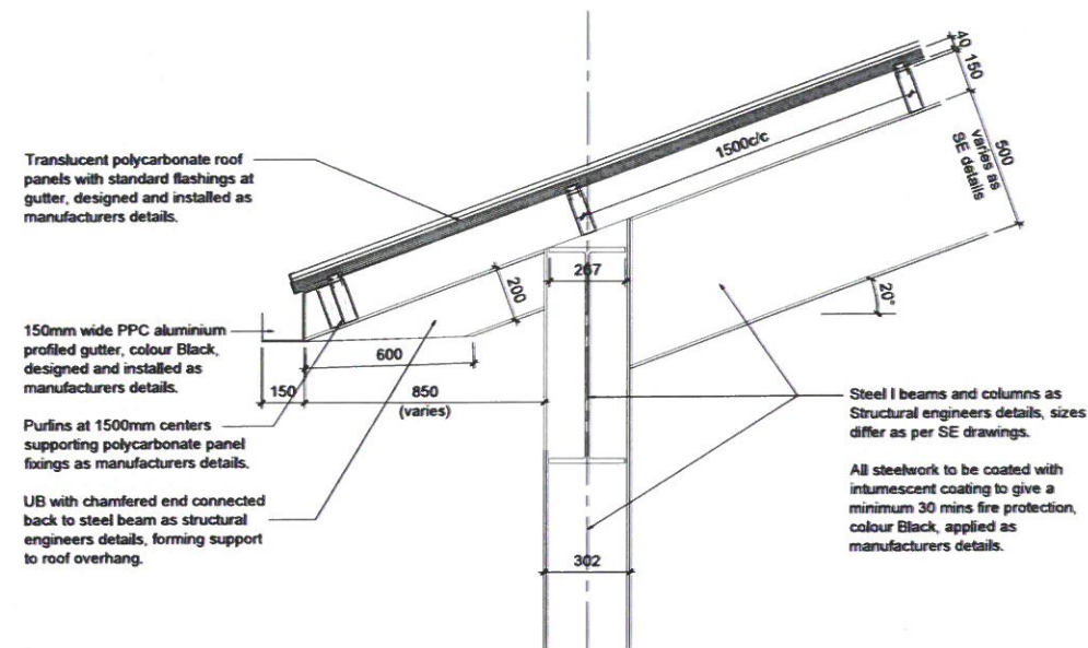
DETAIL 2 POLYCARBONATE PANEL CANOPY ROOF GUTTER DETAIL
