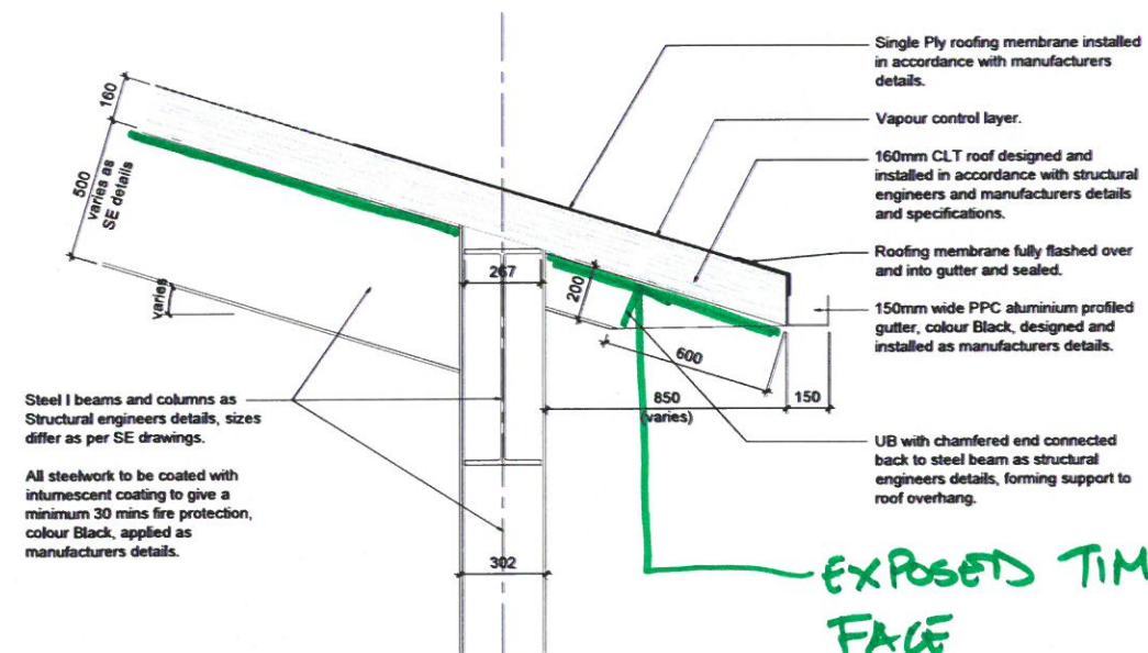
DETAIL 6 SINGLE PLY MEMBRANE CANOPY ROOF GUTTER DETAIL
