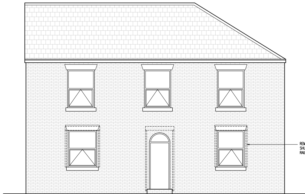
PROPOSED FRONT ELEVATION 1:100 @ A3
