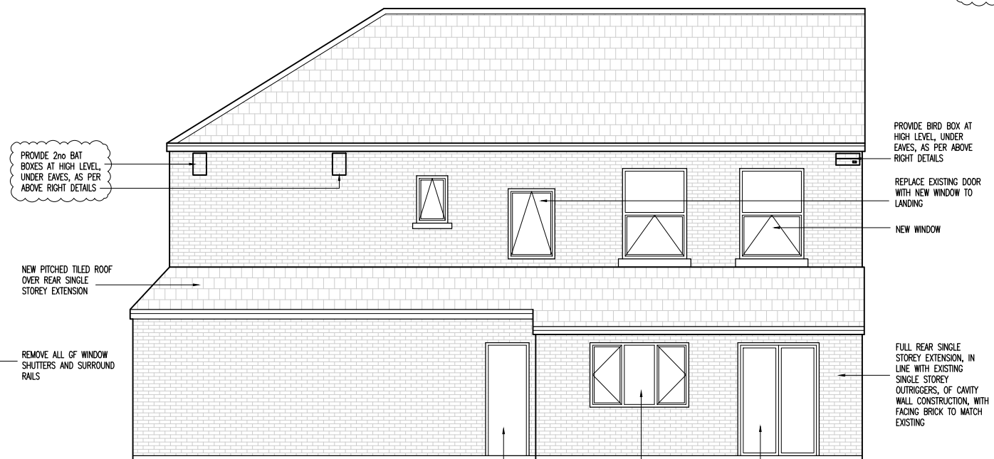
PROPOSED REAR ELEVATION 1:100 @ A3
