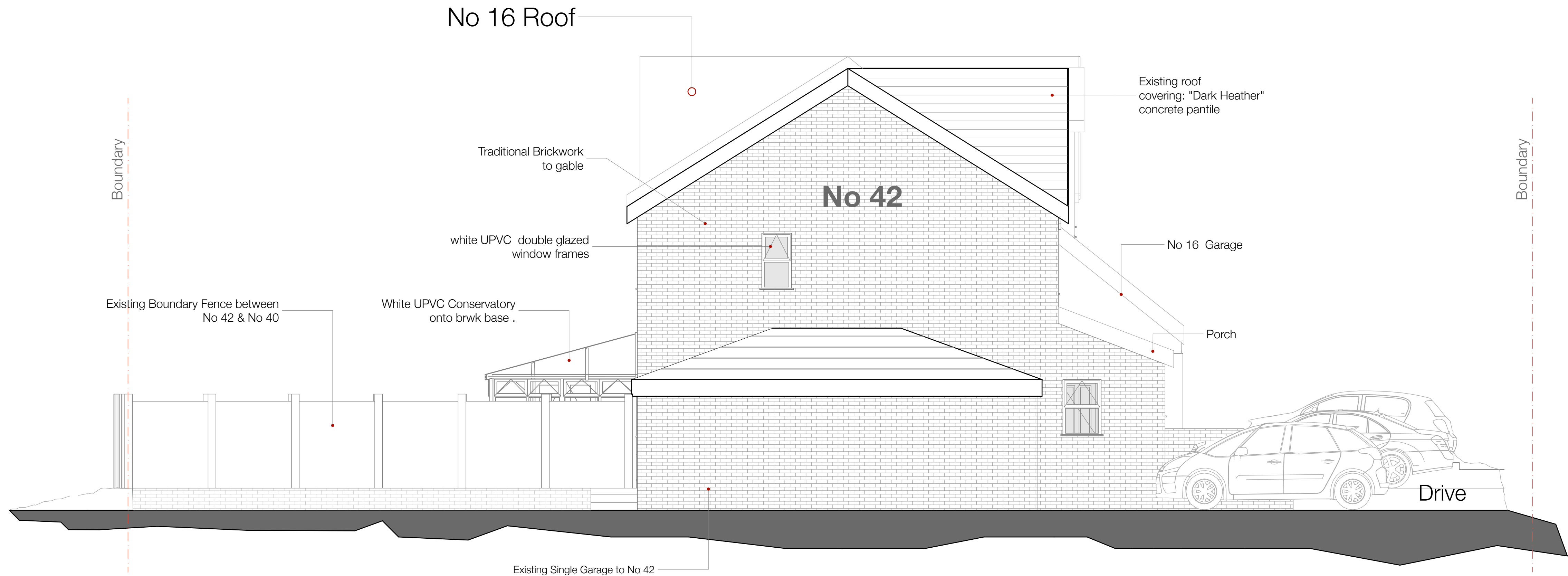
Existing Side Elevation (No 42 - East) scale 1:50 @ A1
