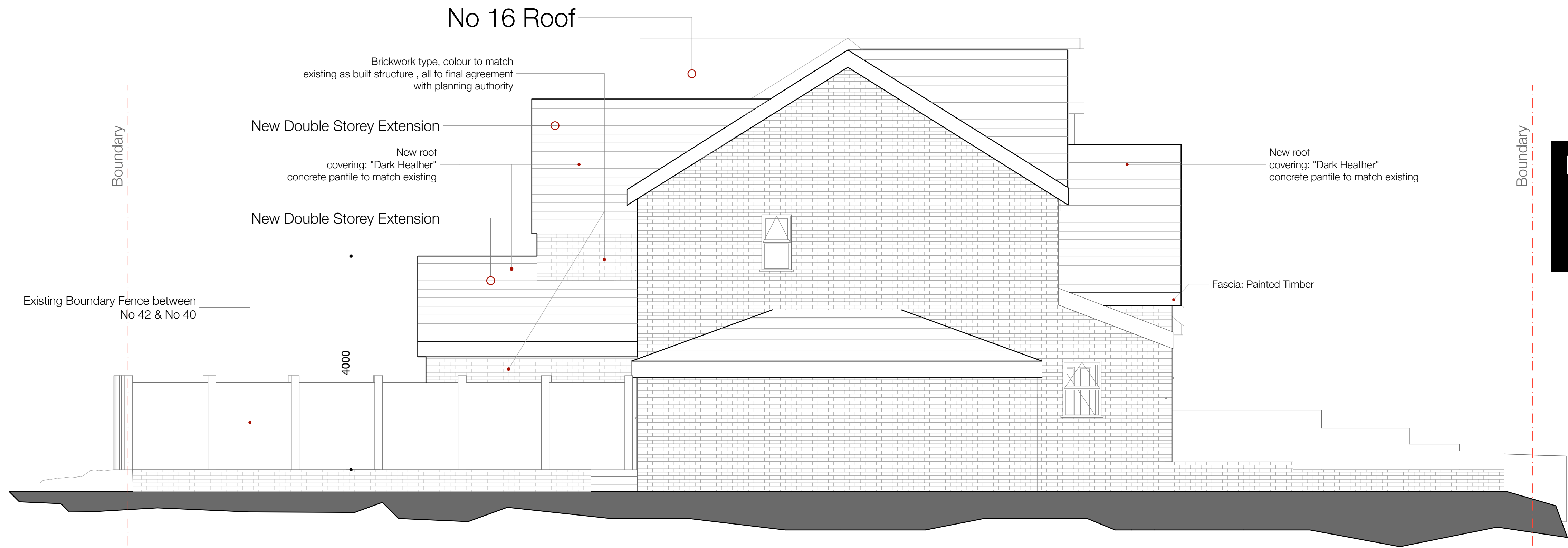
Proposed Side Elevation (No 42 - East) scale 1:50 @ A1
