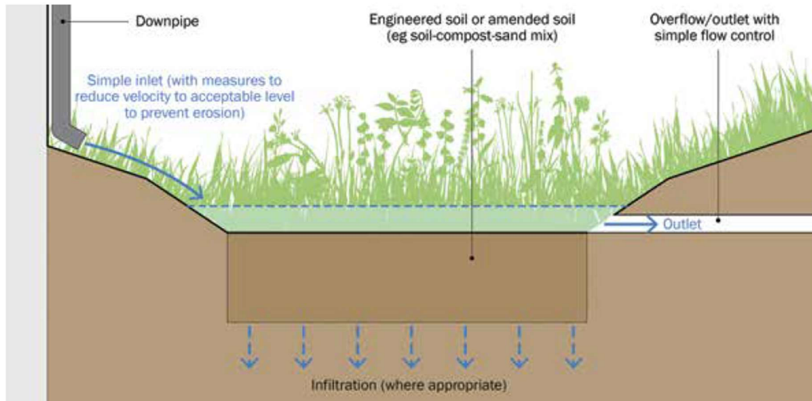
Figure 11 – Typical rain garden (CIRIA, 2015)
