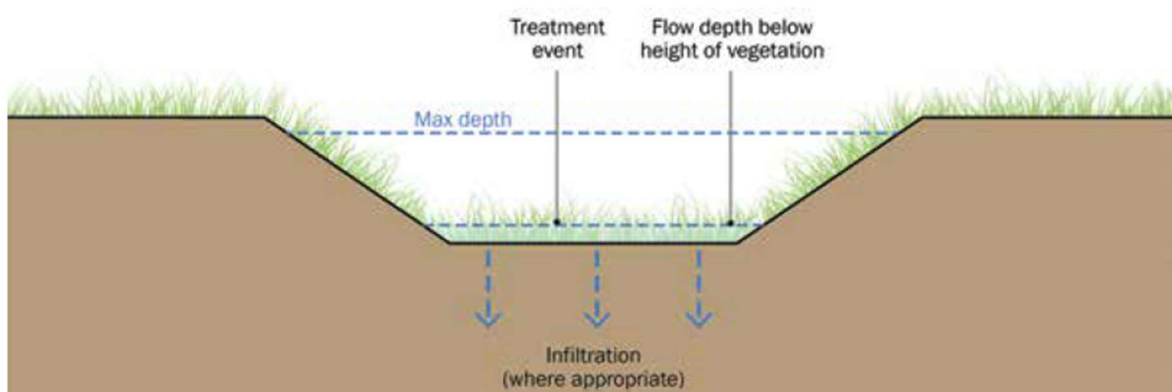
Figure 12 – Typical conveyance/attenuation swale (CIRIA, 2015)
