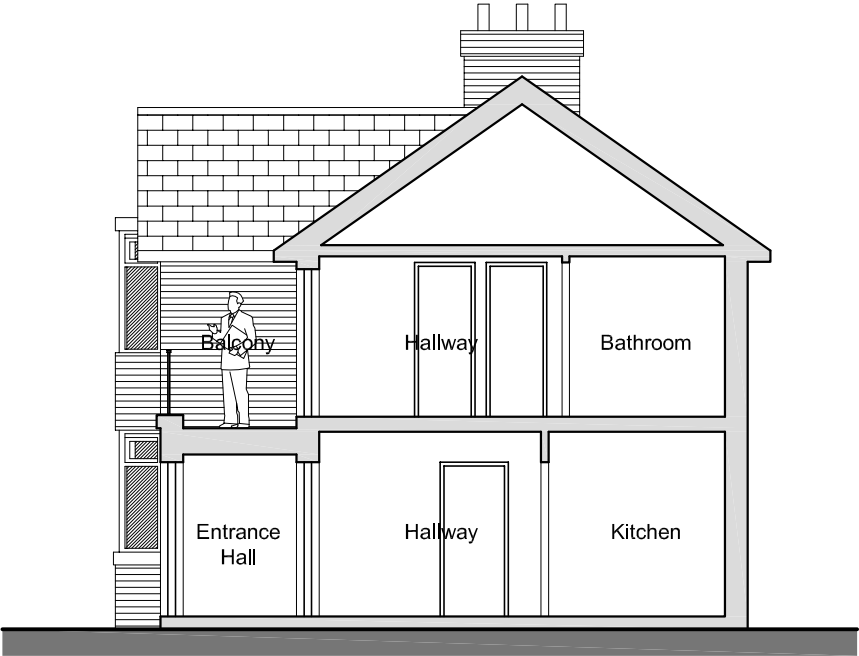
Proposed Side Section A-A 1:100
