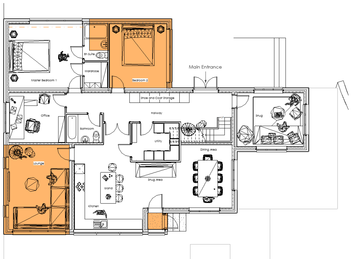
Proposed Ground Floor Plan showing new additions
