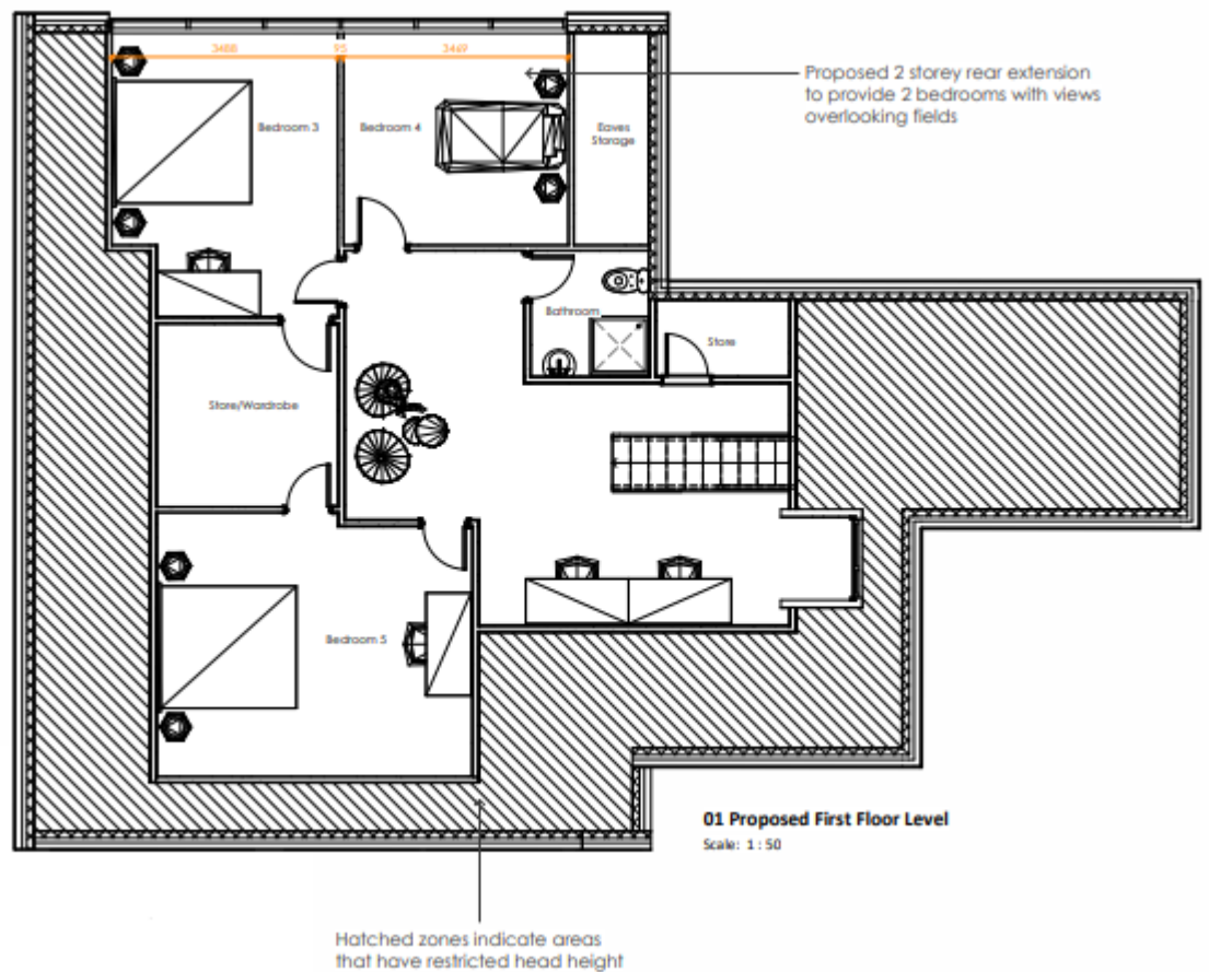
Proposed First Floor Plan showing new additions
