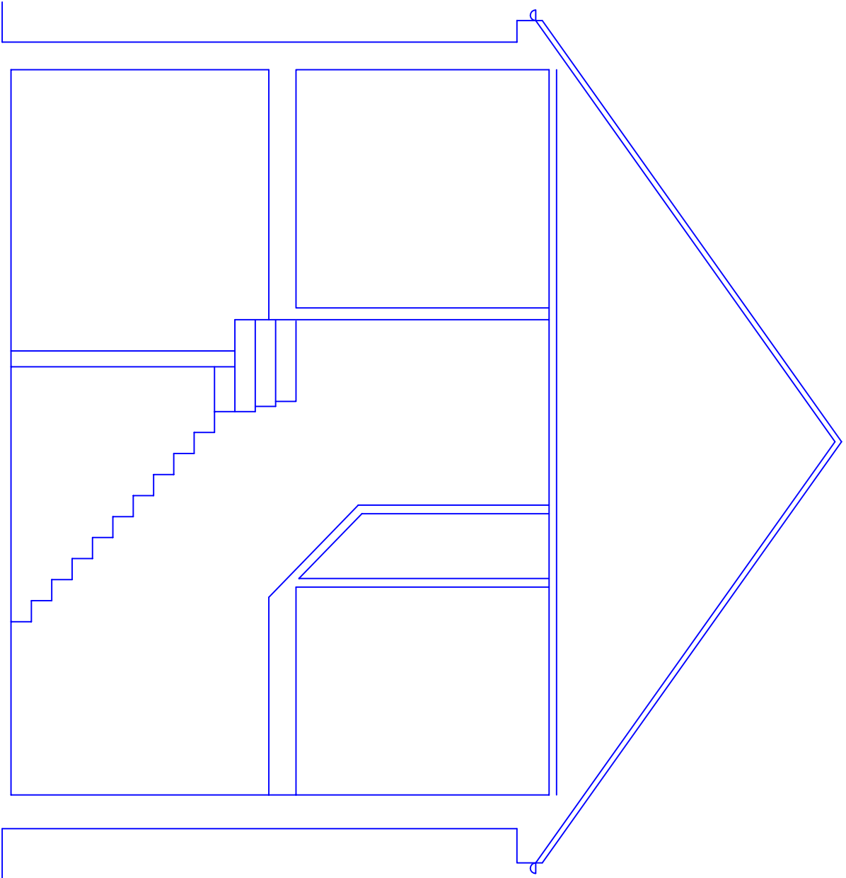
Existing Section
