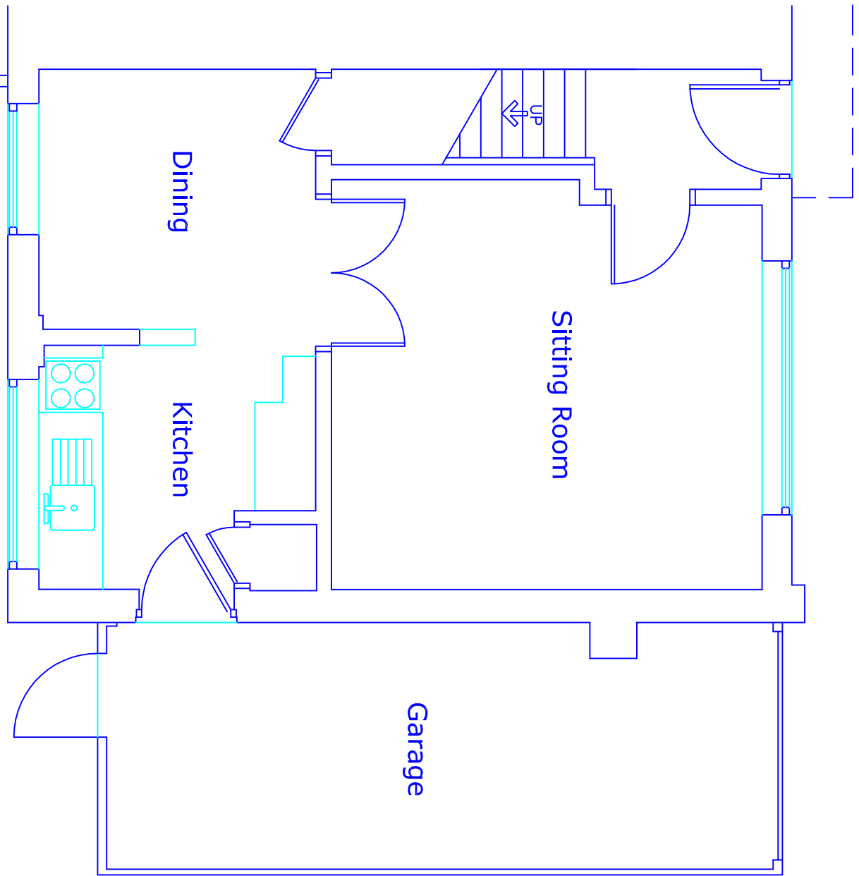
Existing Plan Ground Floor
