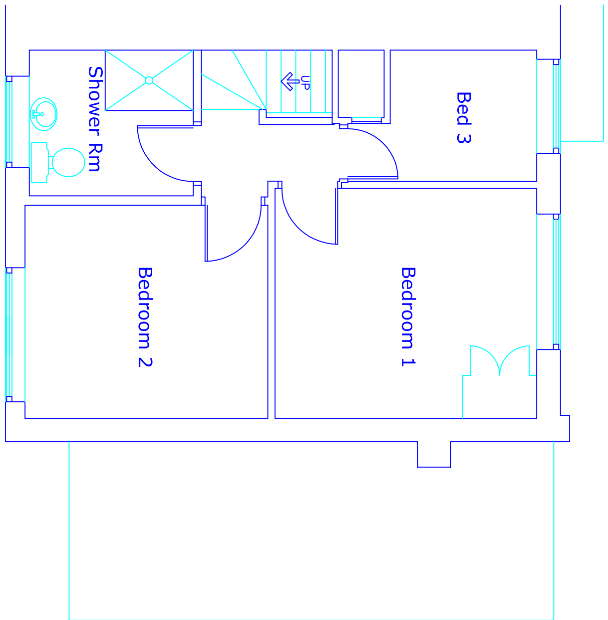
Existing Plan First Floor
