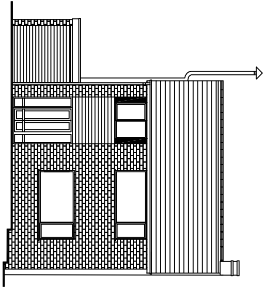
FRONT ELEVATION (EXISTING)
