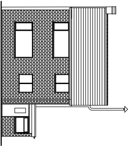
REAR ELEVATION (EXISTING)
