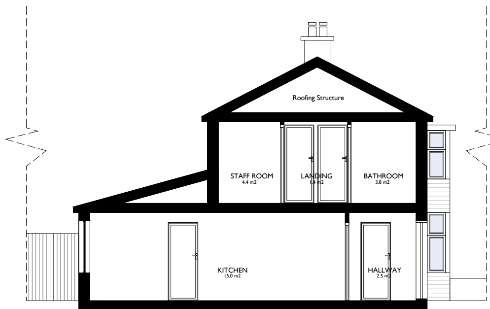
Proposed AA Section
