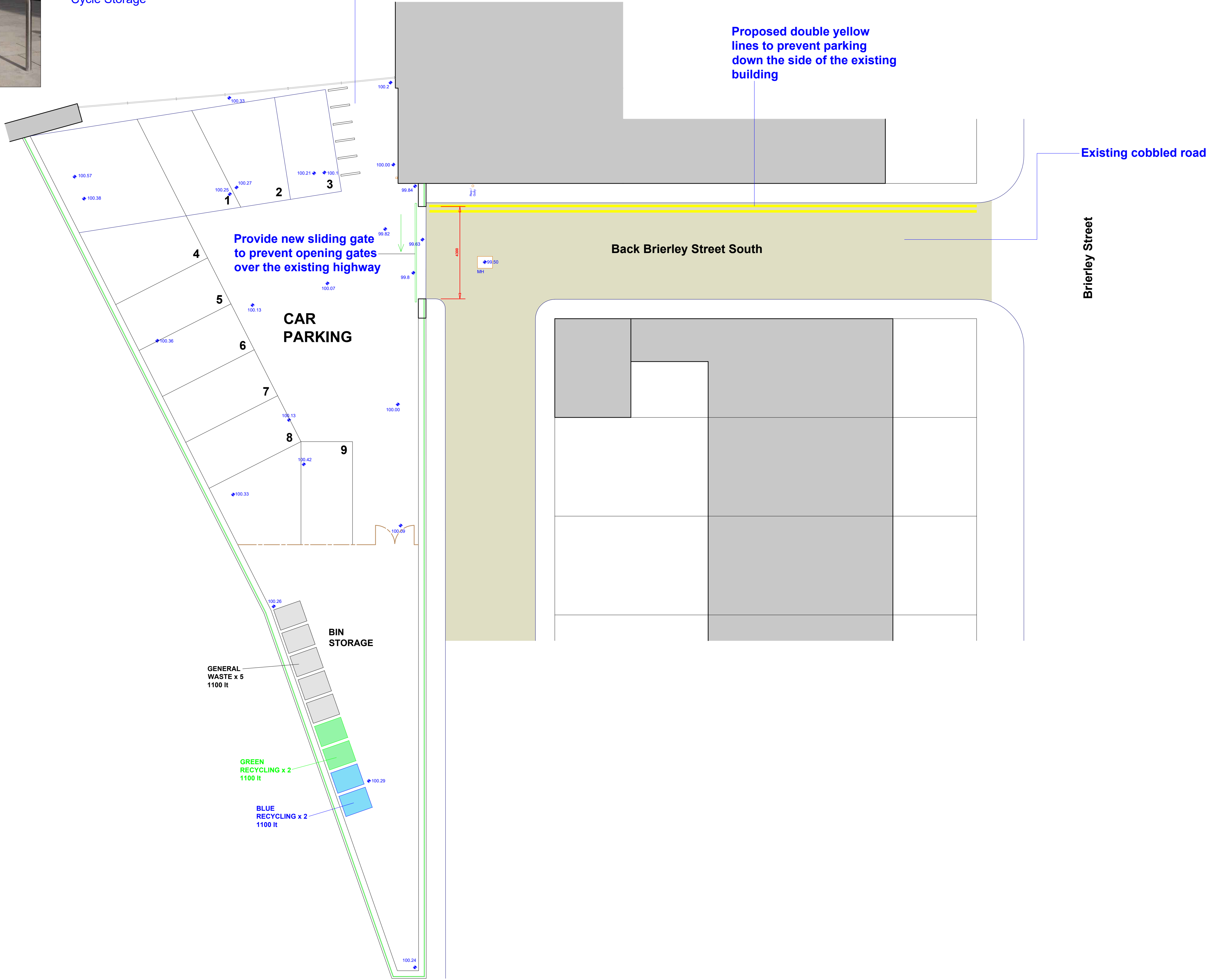
PROPOSED CAR PARK PLAN
