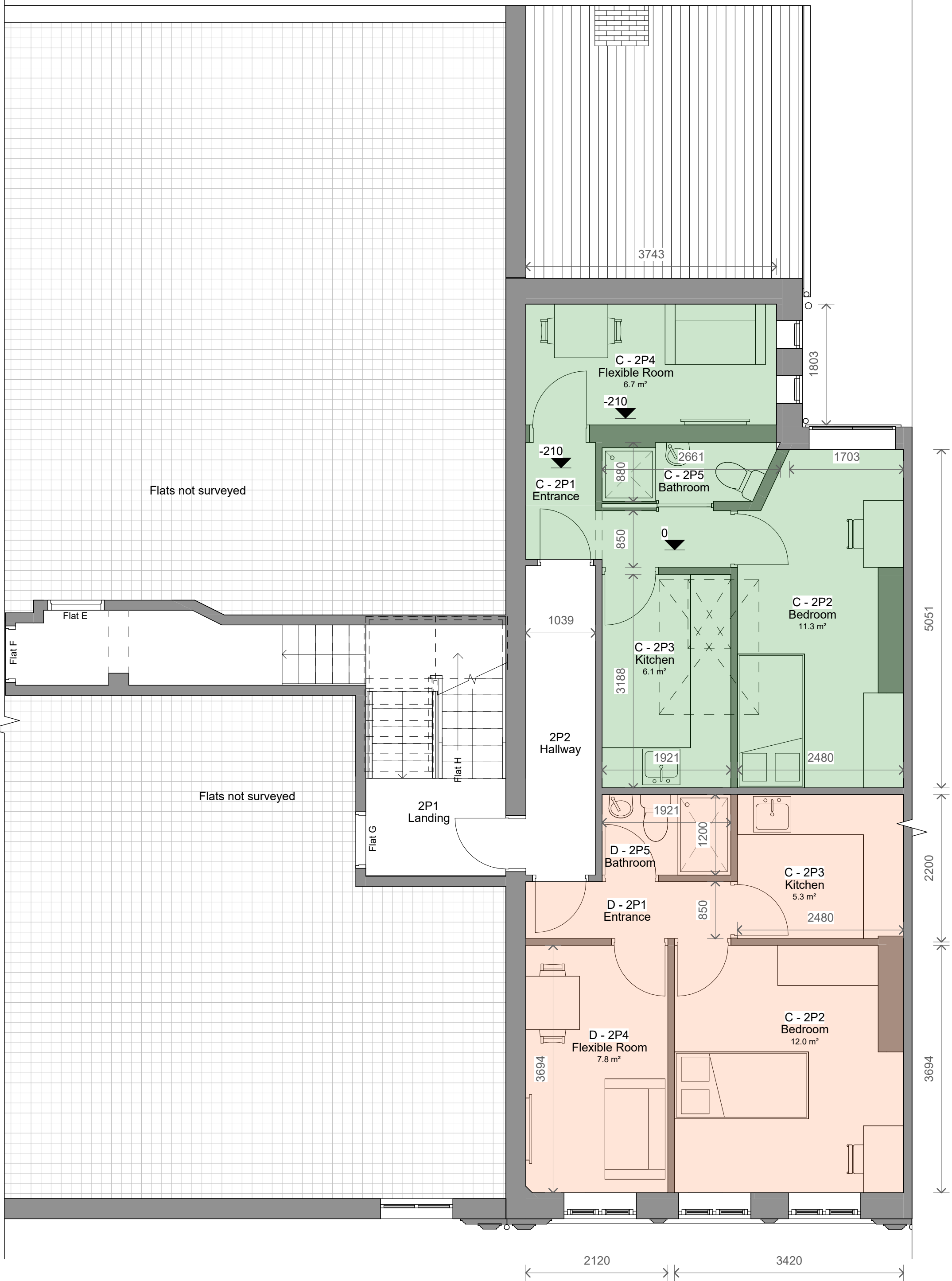
2 Level 2 - Proposed 1 : 50
