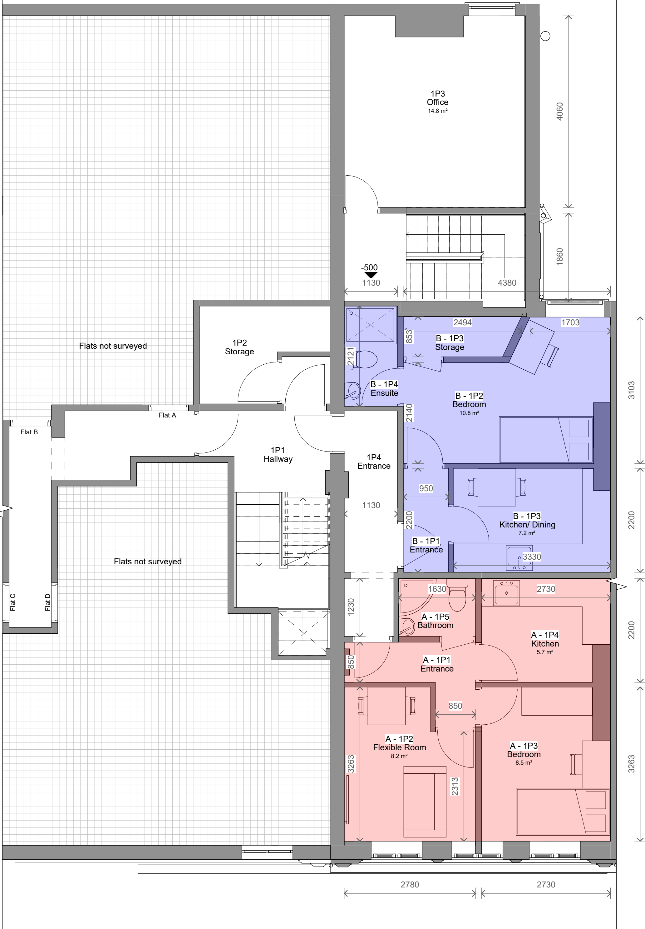
1 Level 1 - Proposed 1 : 50
