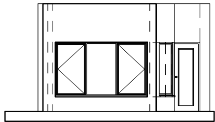
PROPOSED FRONT ELEVATION
