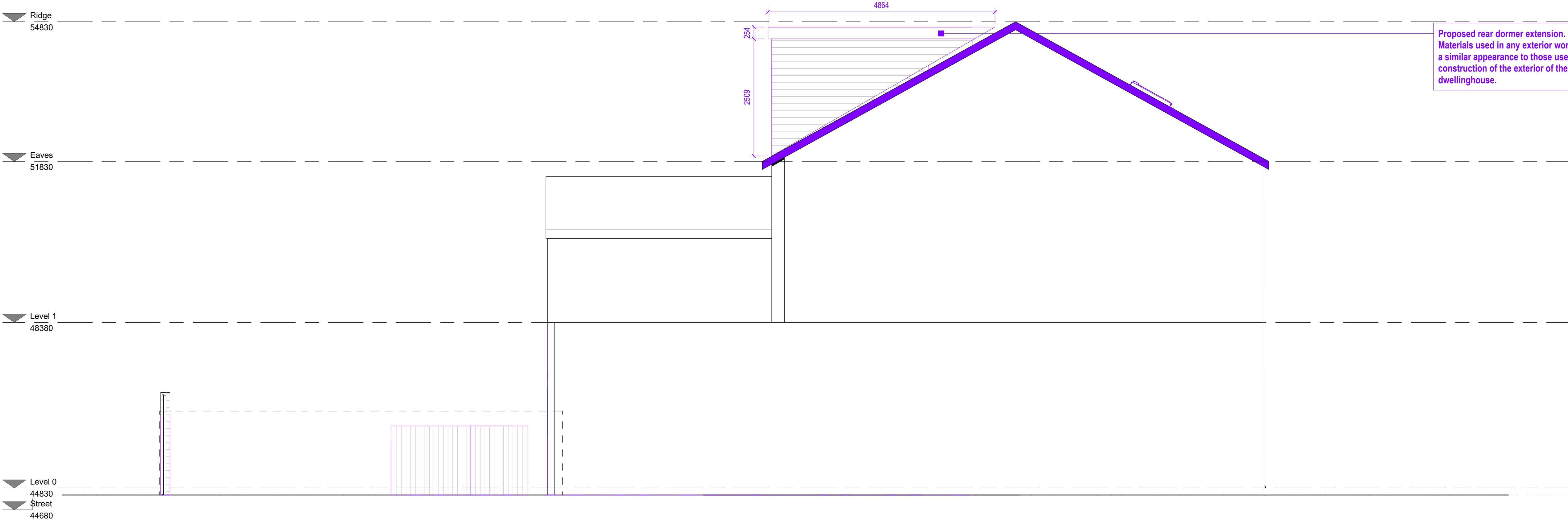
2 Proposed Side 1 Elevation 1 : 50
