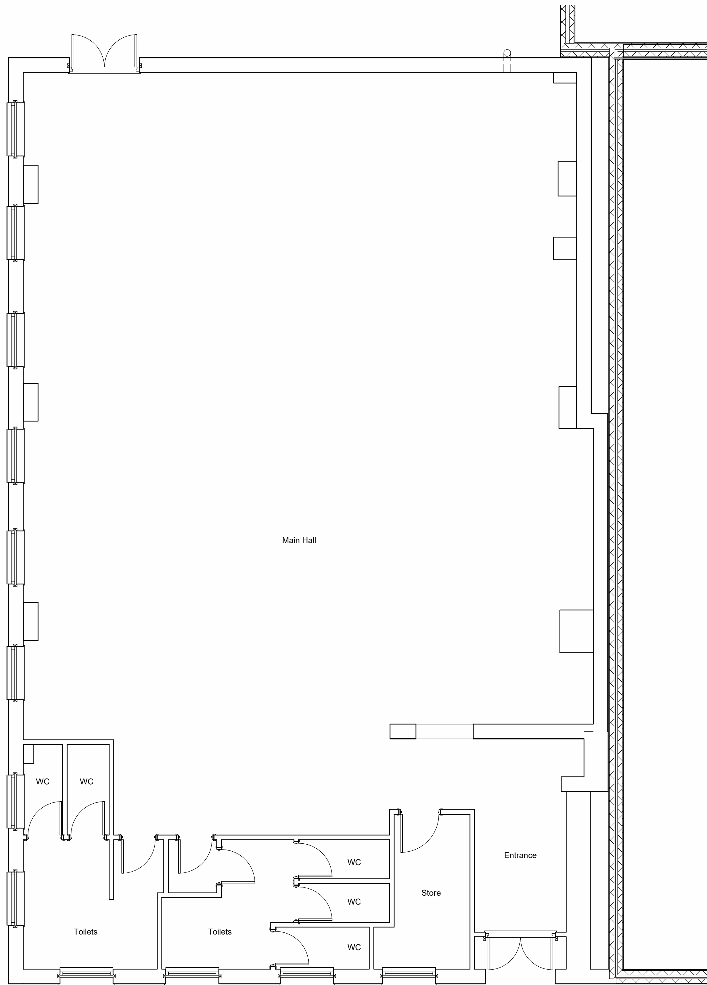
Existing GF Plan 1 : 50
