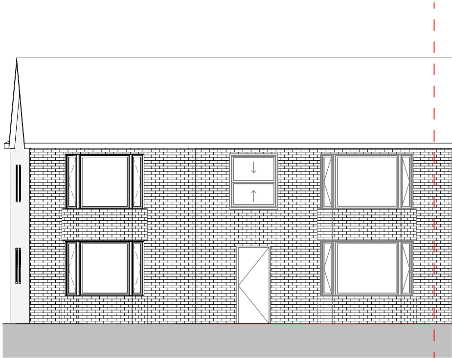
Front Elevation as Proposed 1 : 100
