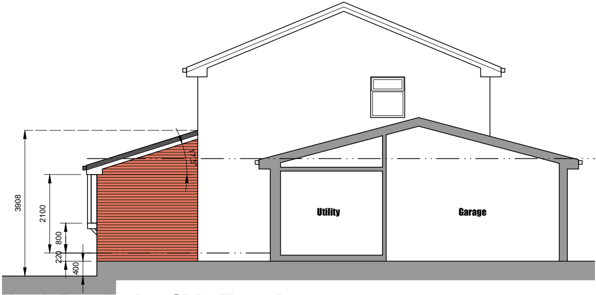
North East Facing Side Elevation
