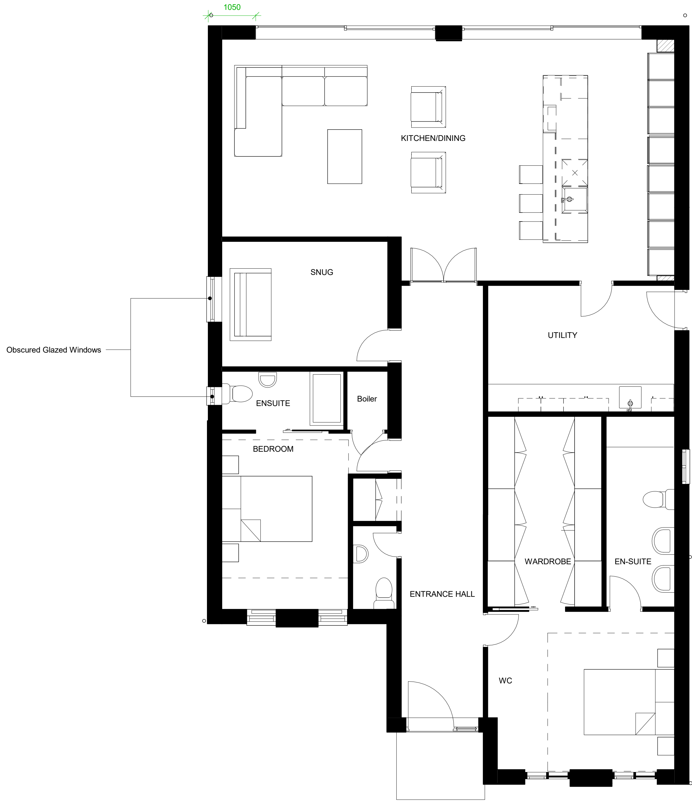
1. Level 0 GA Proposed 1 : 50
