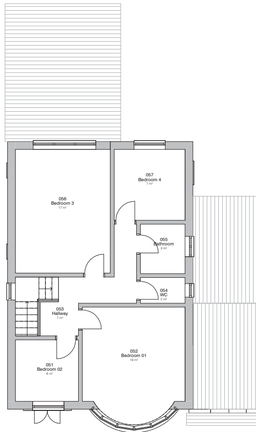
6. Level 1 - GA Existing 1:50
