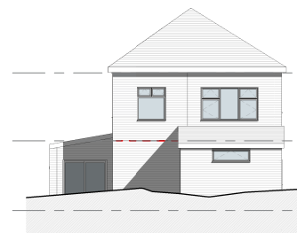
3. Rear - Existing 1:100
