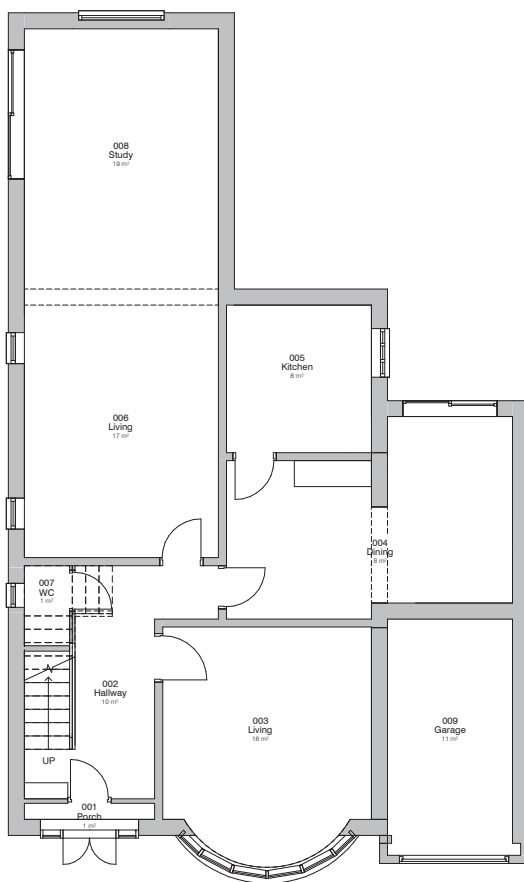
5. Level 0 - GA Existing 1:50
