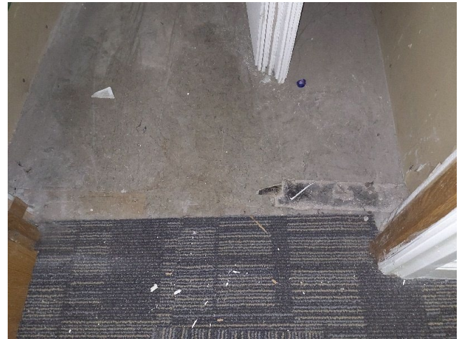
Sample No: Refer to Sample 23/4/B/18/JPS5 G.04 Understairs Store Floor Area Below Floor Screed Vinyl Floor Tiles and Bitumen Adhesive No Asbestos Detected
