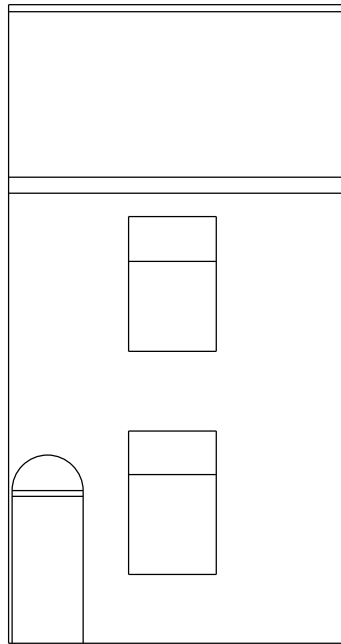
EAST ELEVATION
