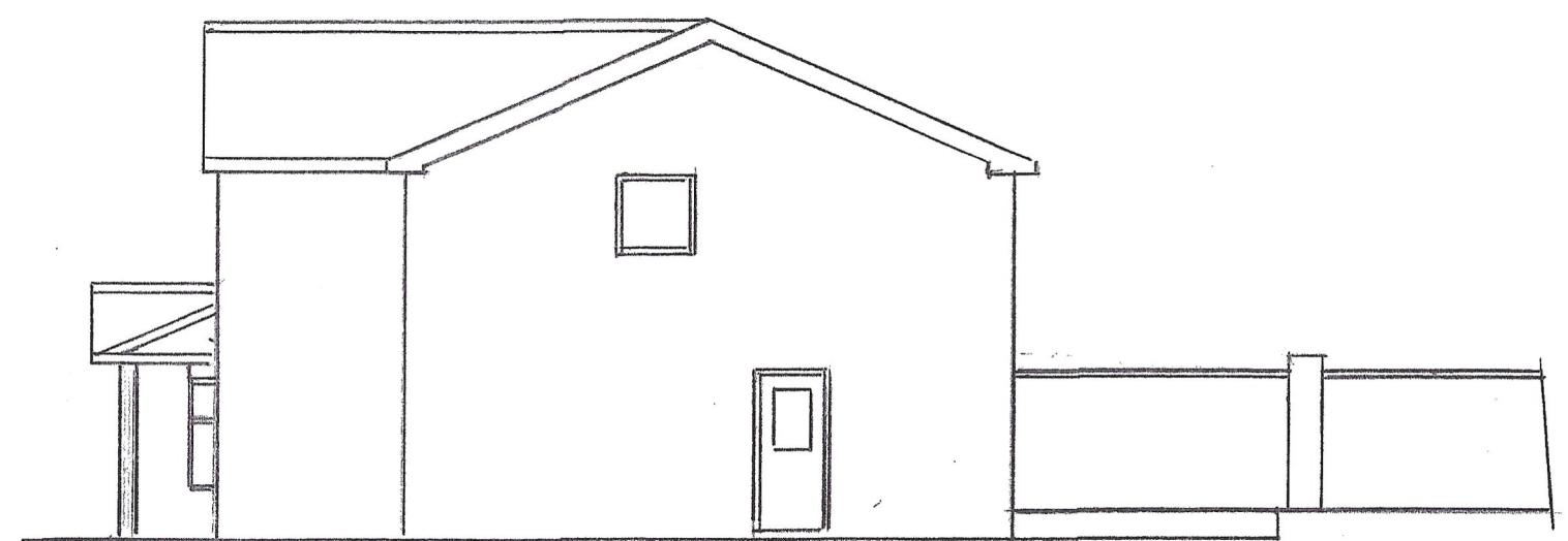
SIDE ELEVATION
