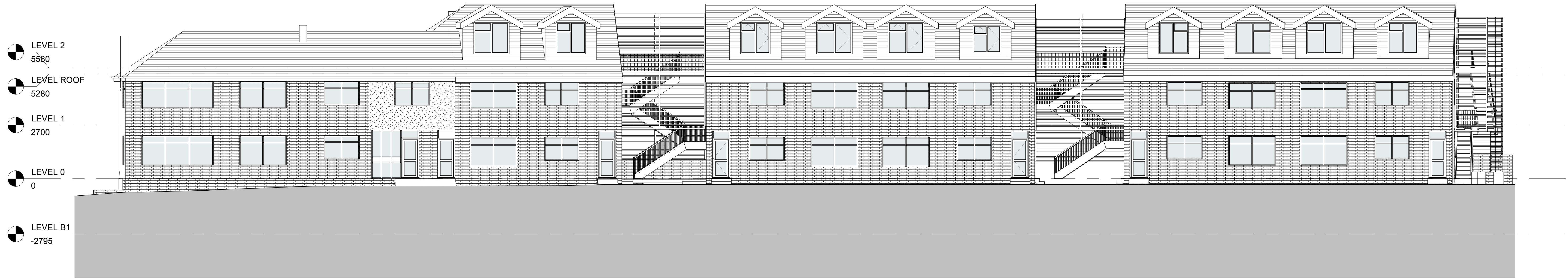
1 Front - Proposed 1 : 100
