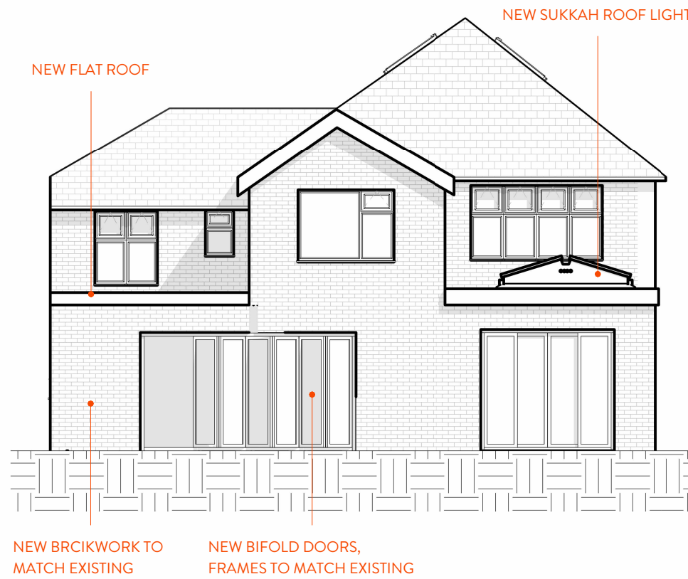
5 South - Proposed 1 : 100
