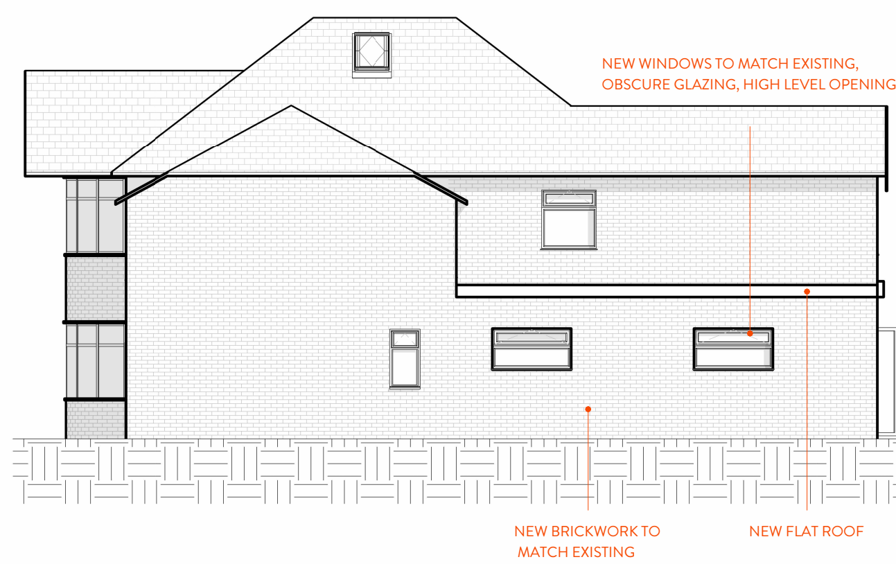
6 West - Proposed 1 : 100
