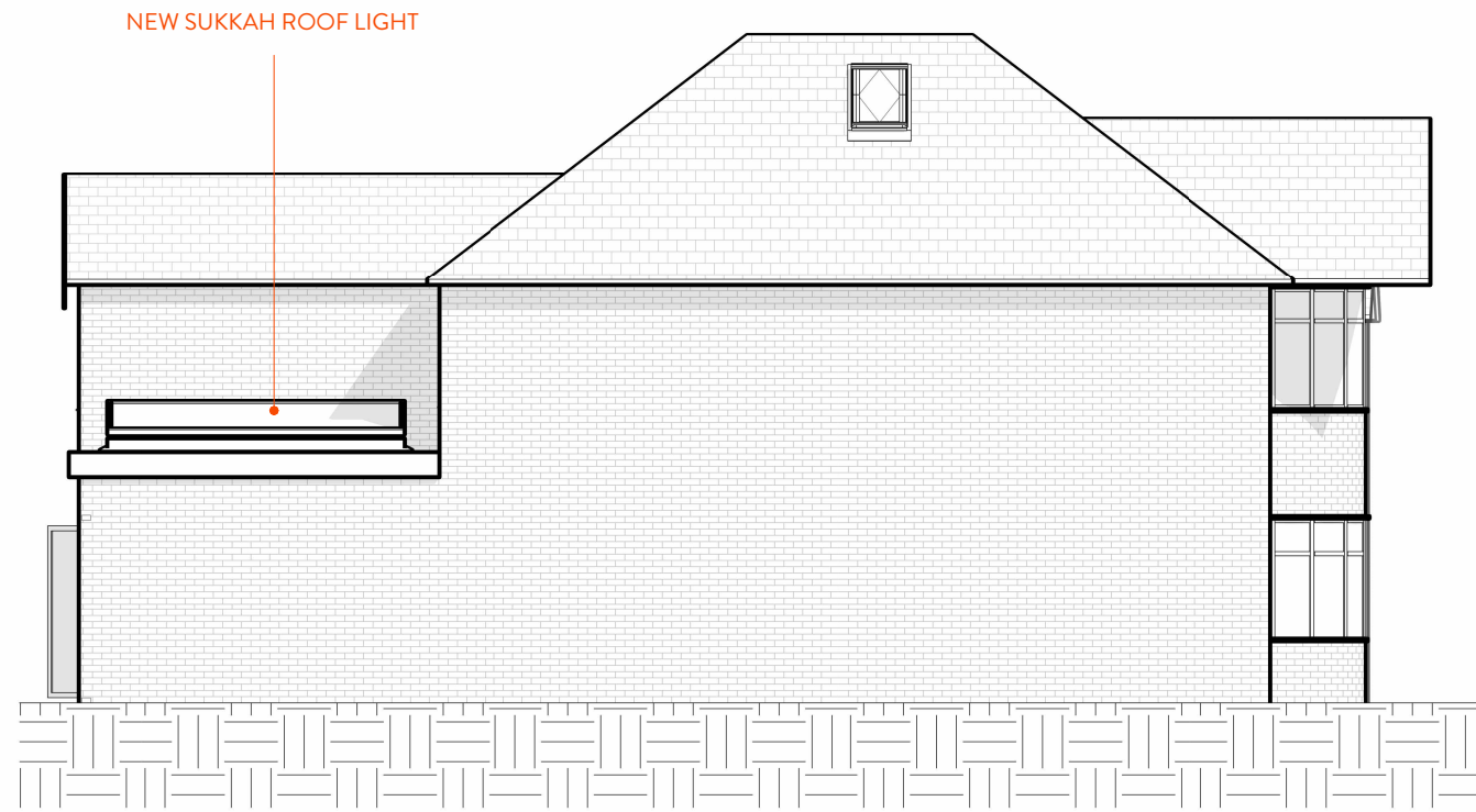
3 East - Proposed 1 : 100
