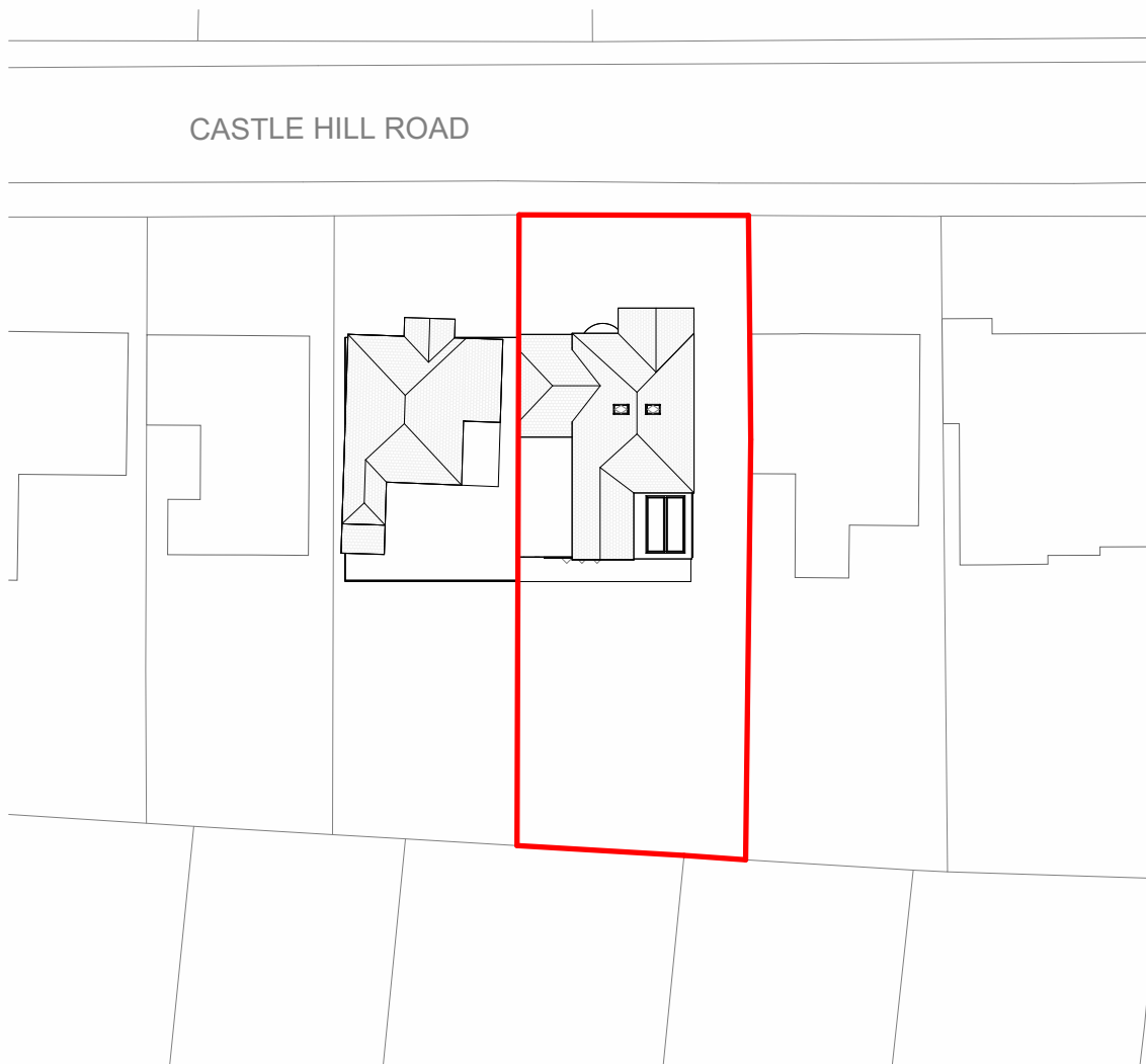
7 Block Plan - Proposed 1 : 500
