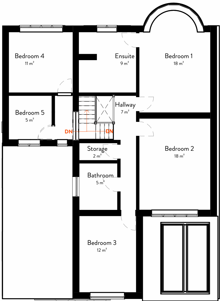
2 First Floor - Proposed 1 : 100
