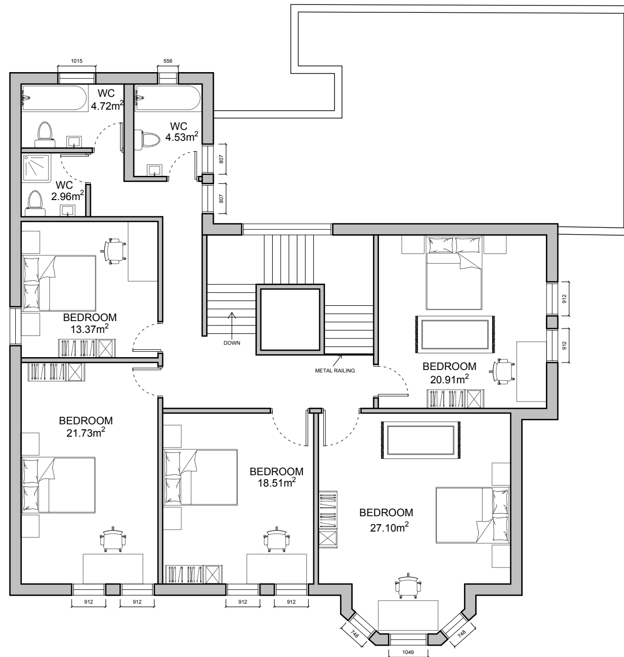
Proposed First Floor Plan Revision 1
