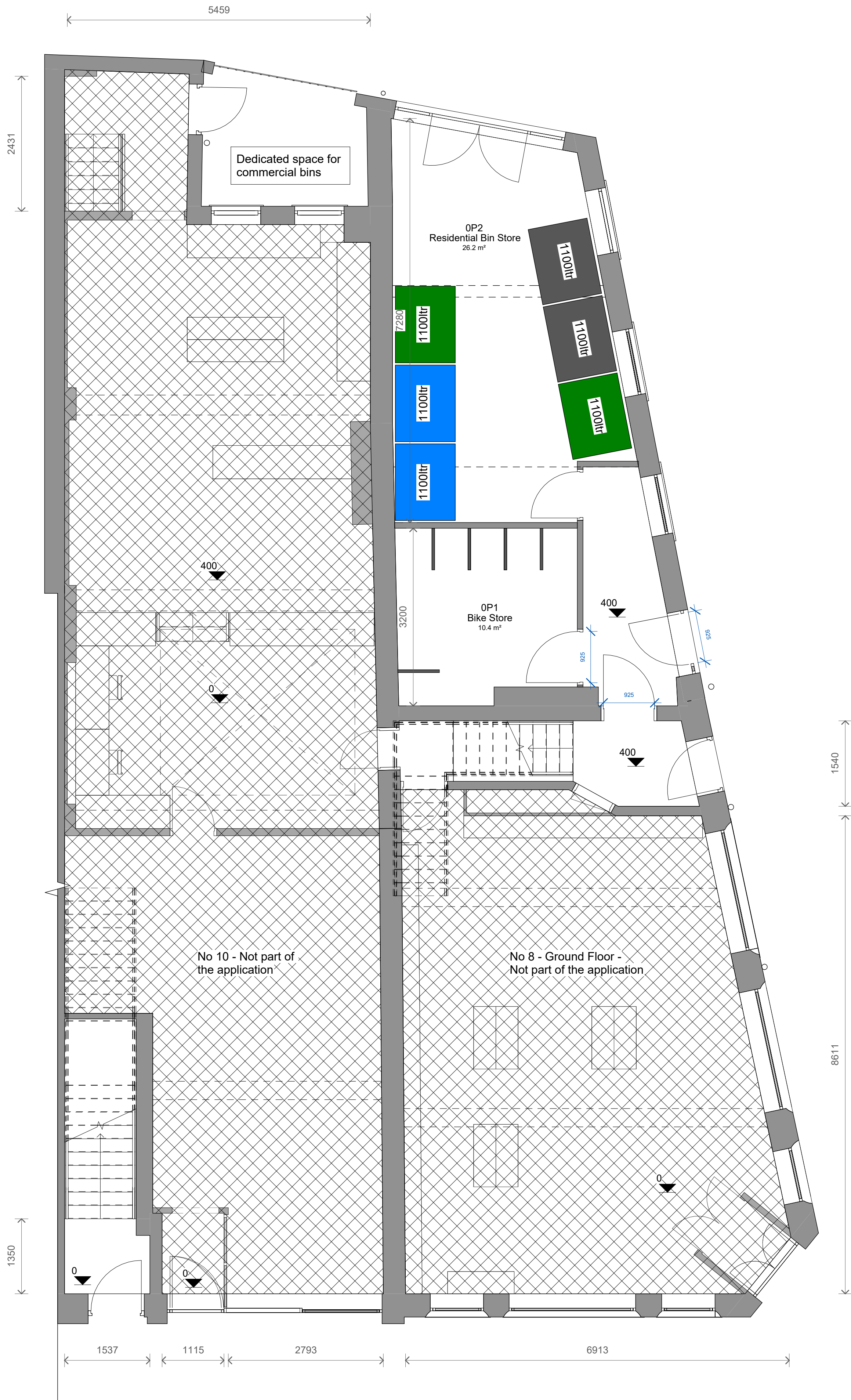
1 Level 0 - Proposed 1 : 50
