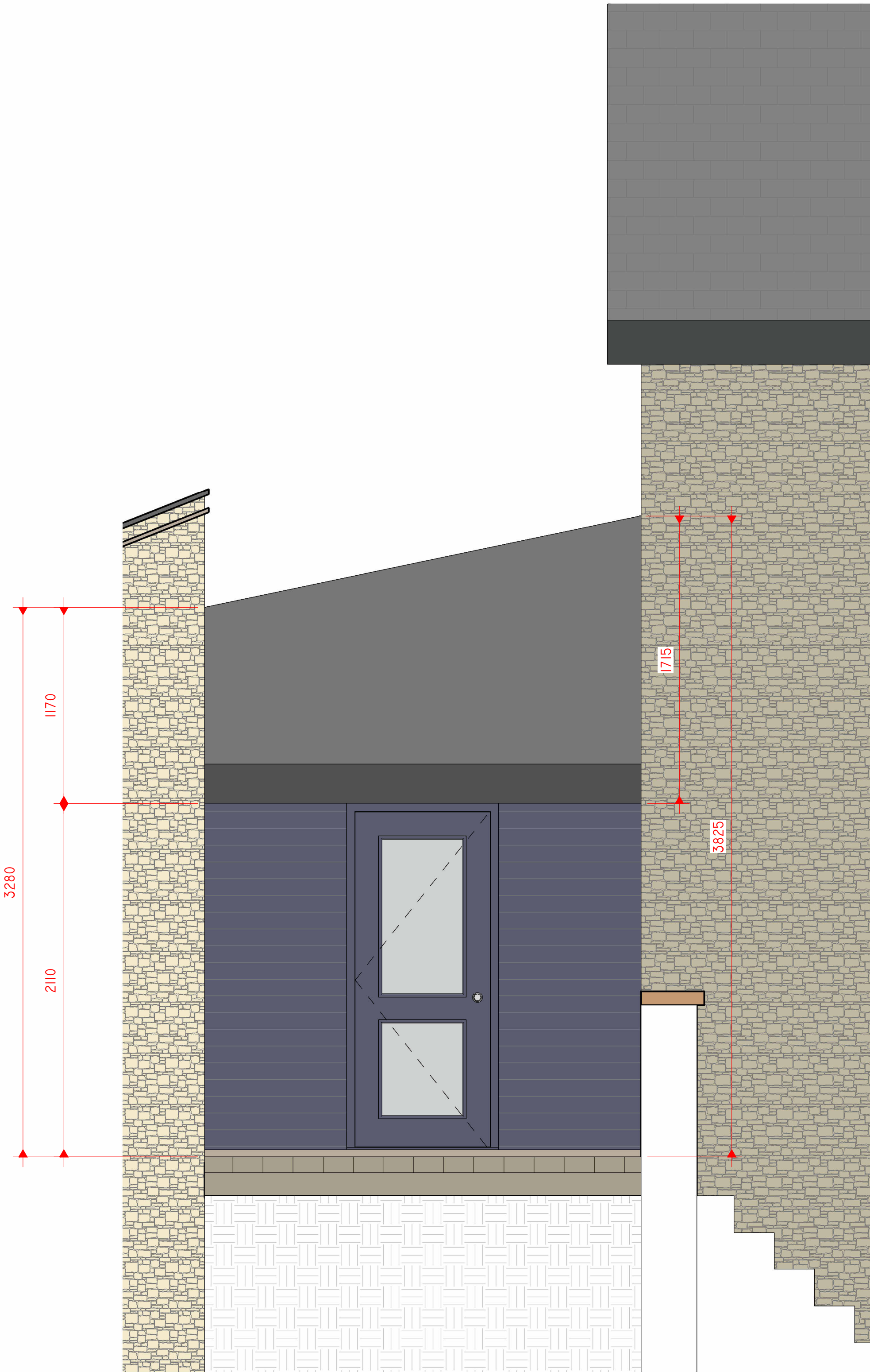
EXISTING PORCH ELEVATION
