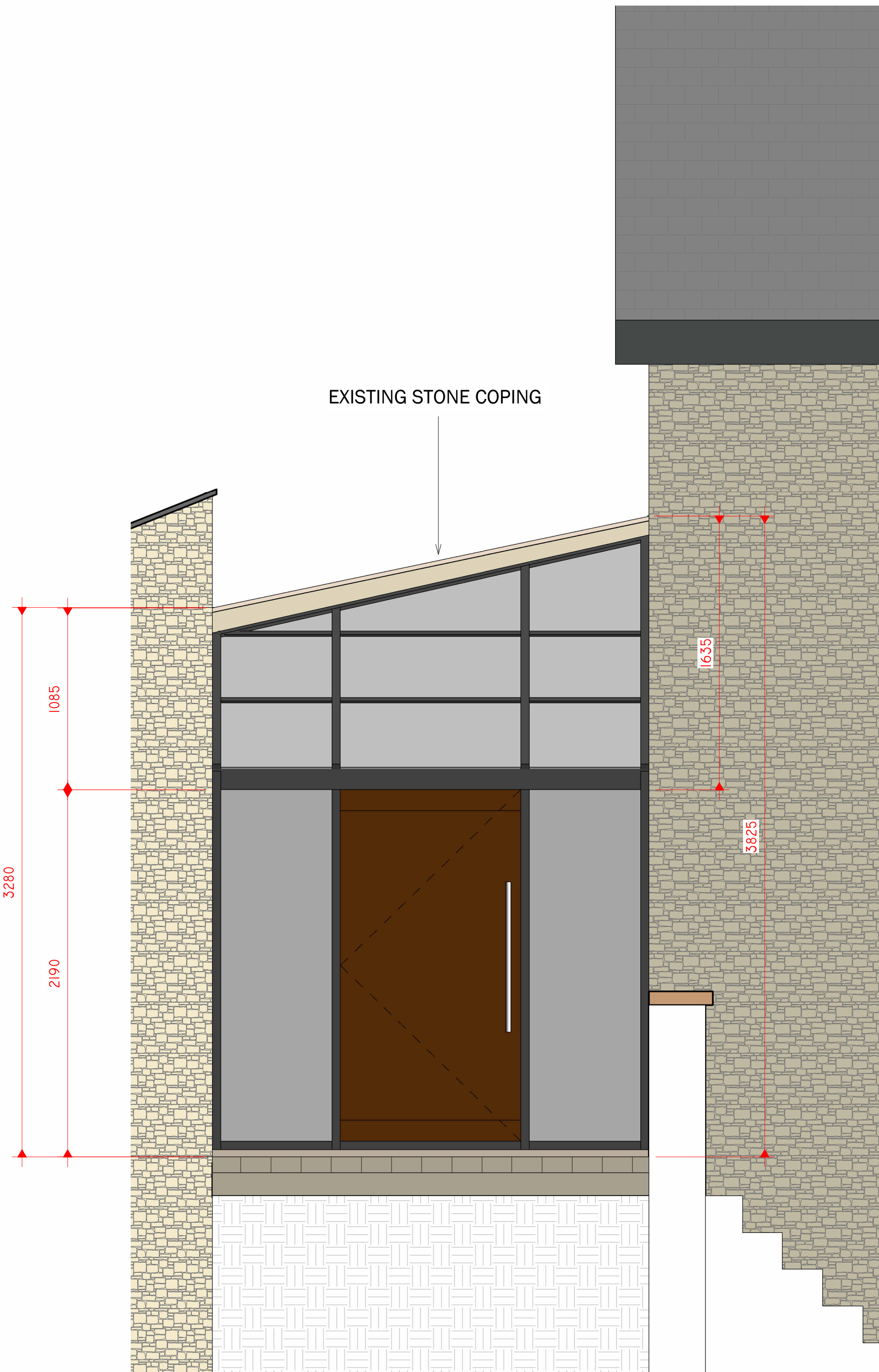
PROPOSED PORCH ELEVATION
